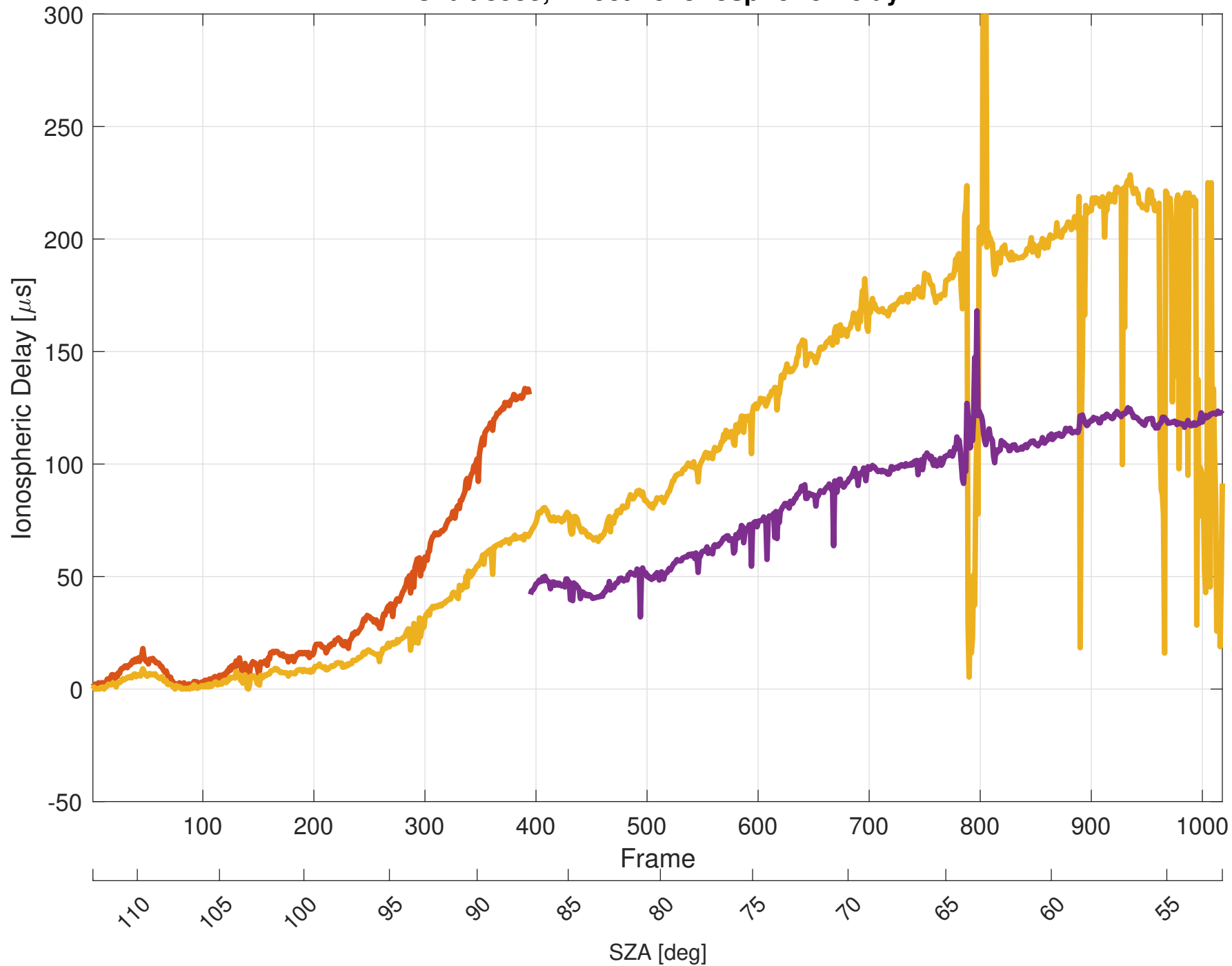
Orbit 8538, Effective Ionospheric Delay
