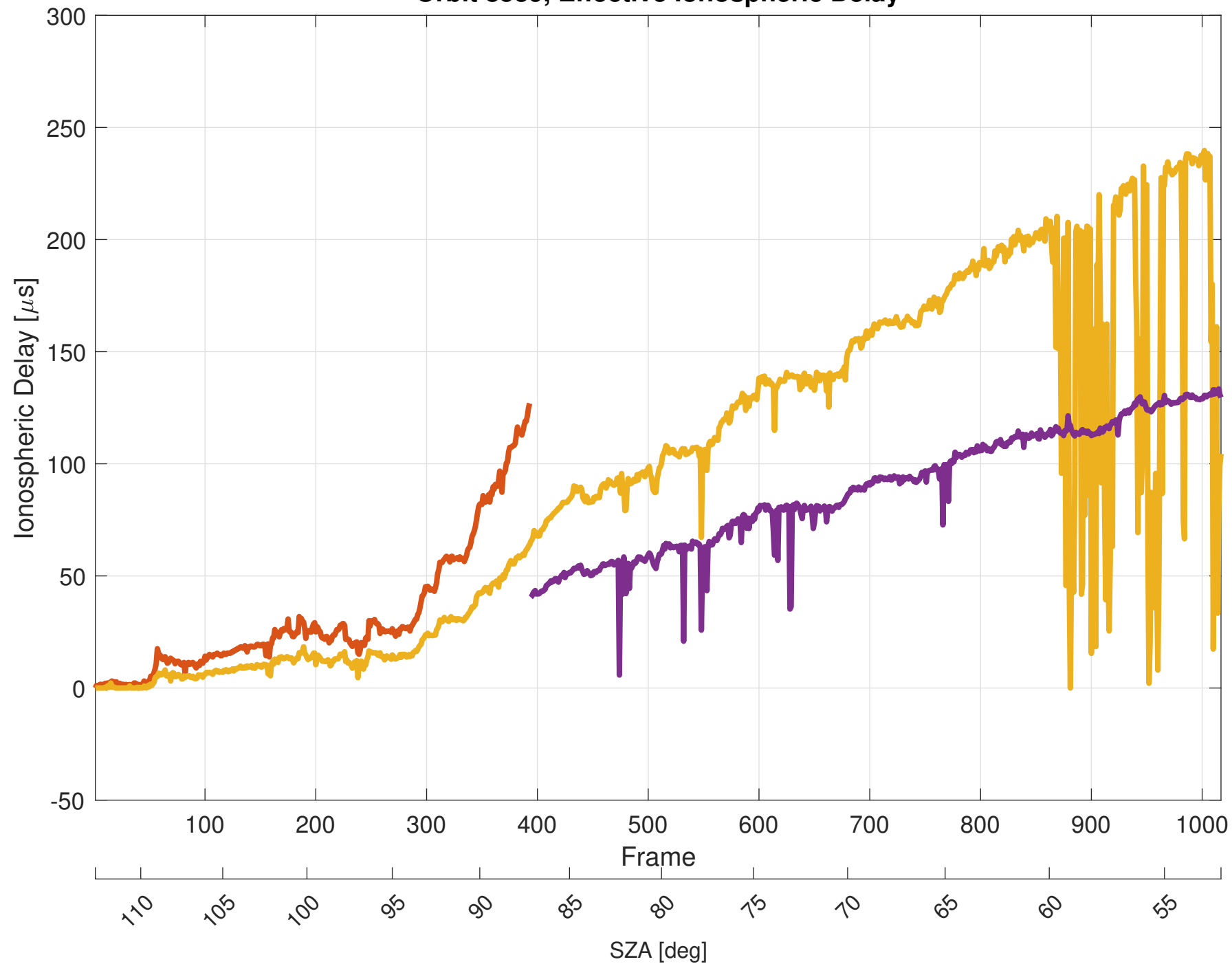
Orbit 8539, Effective Ionospheric Delay
