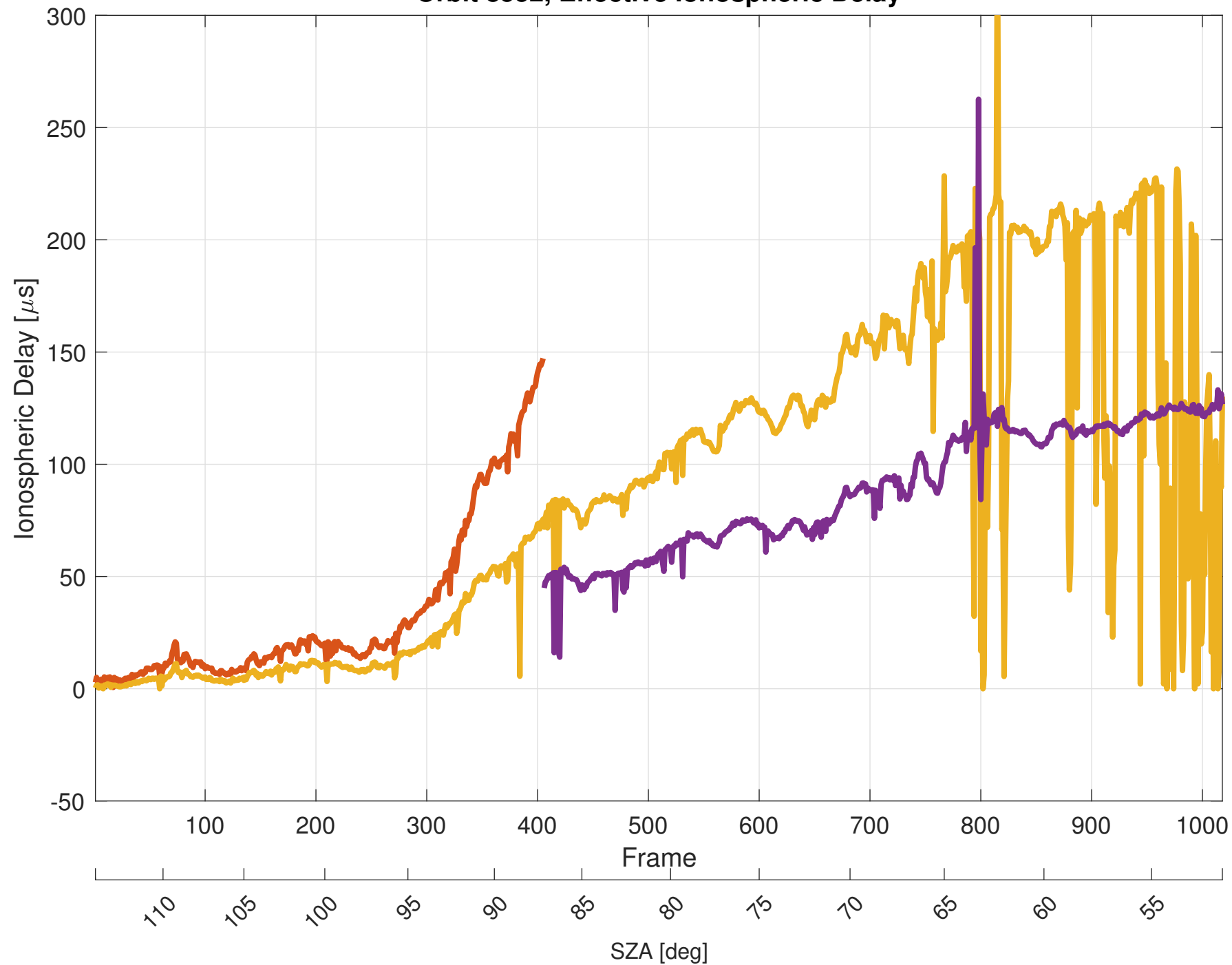
Orbit 8552, Effective Ionospheric Delay
