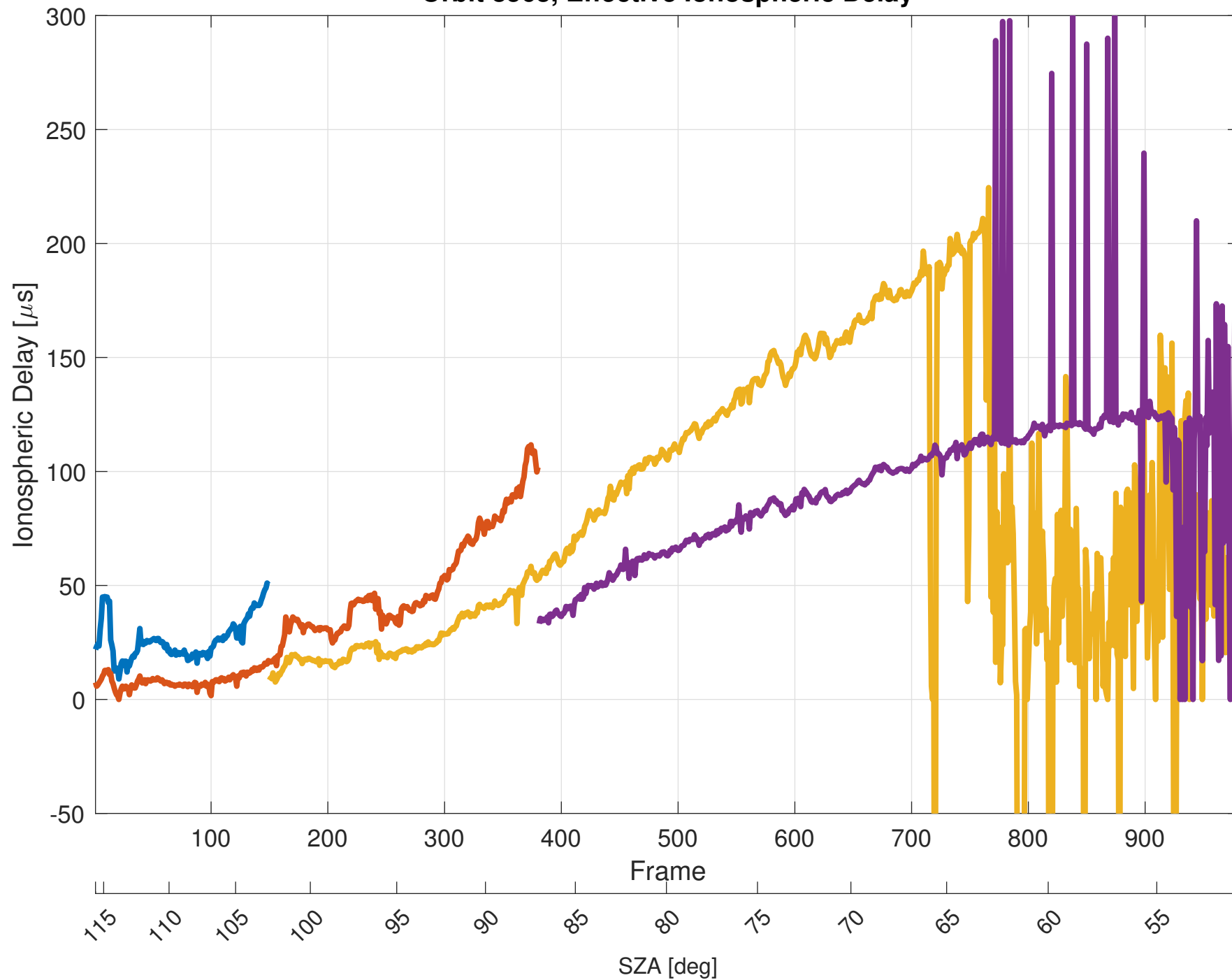
Orbit 8563, Effective Ionospheric Delay
