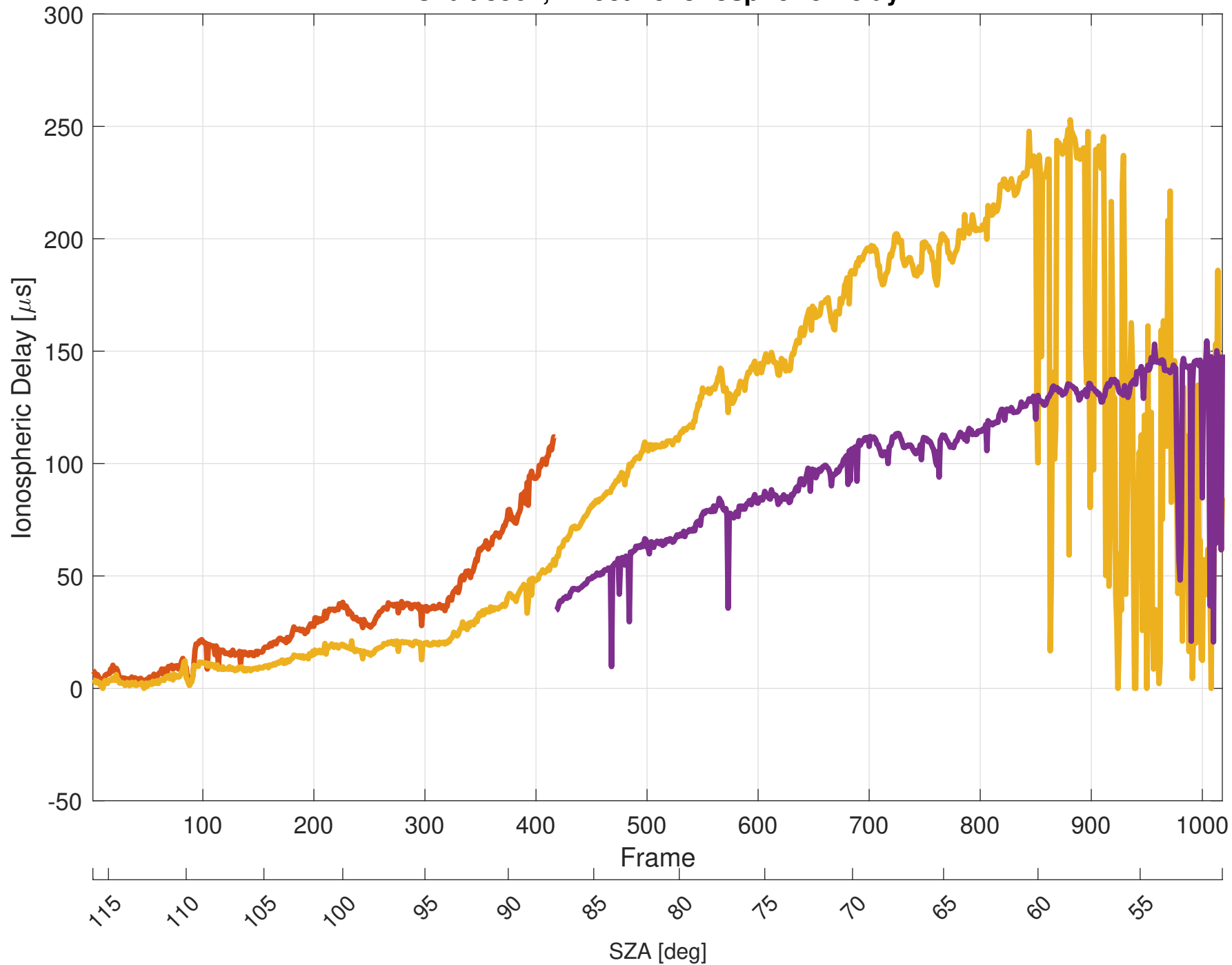
Orbit 8567, Effective Ionospheric Delay
