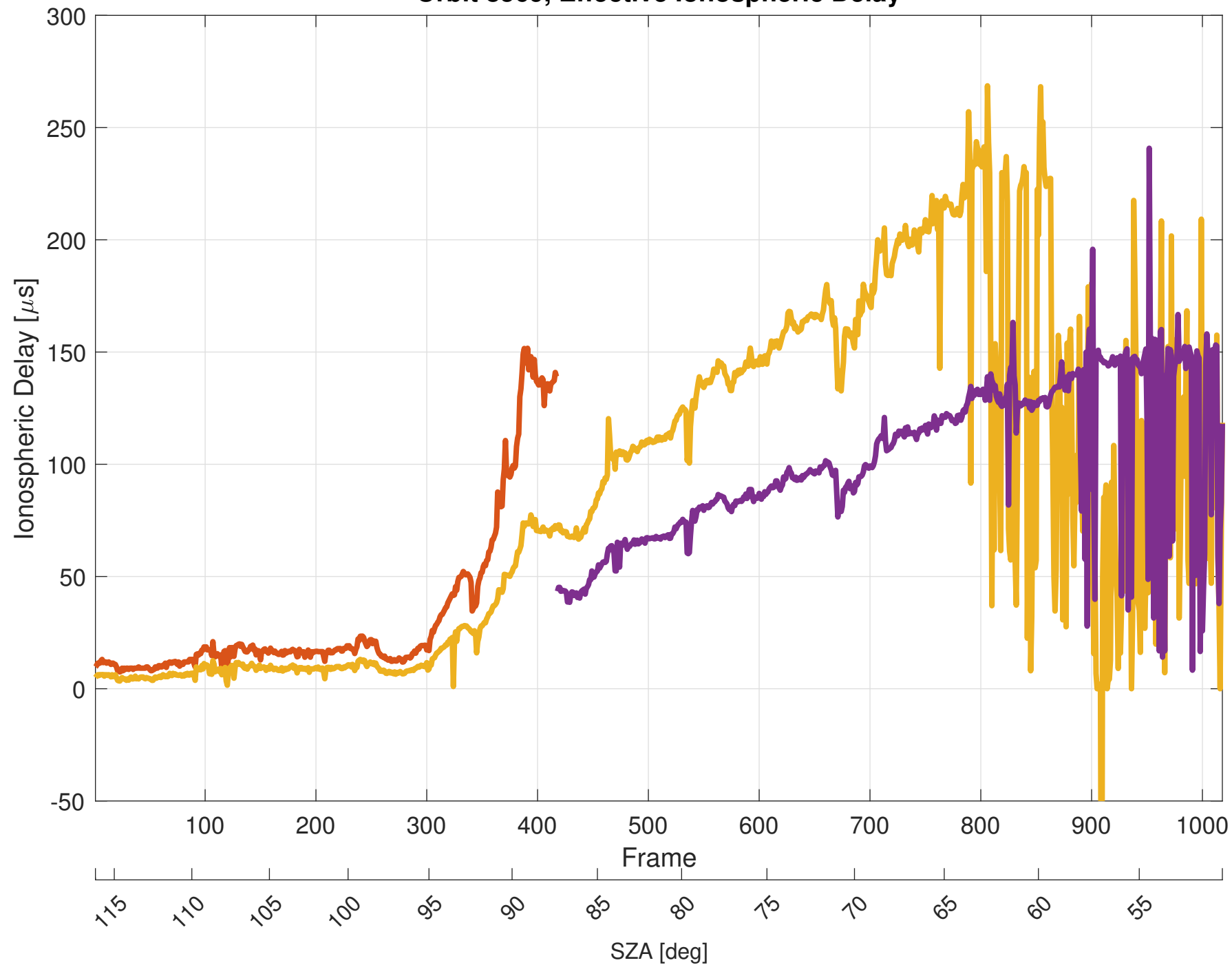
Orbit 8569, Effective Ionospheric Delay
