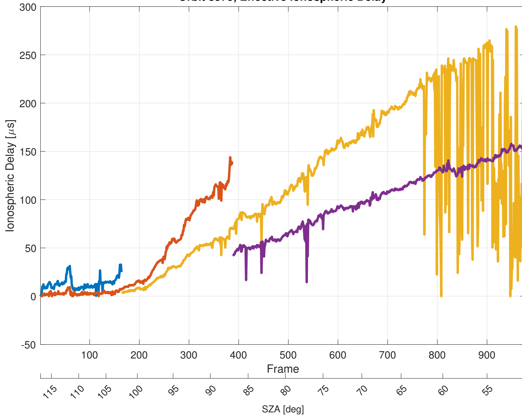
Orbit 8575, Effective Ionospheric Delay
