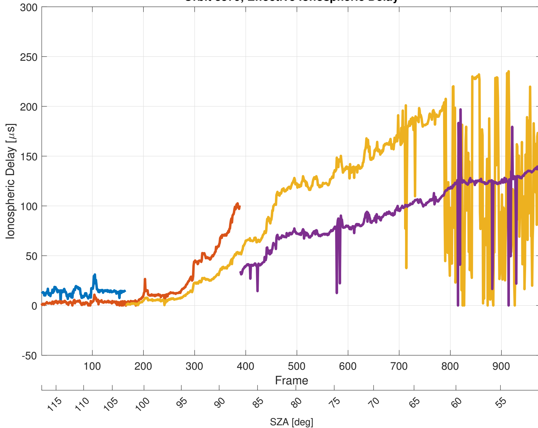
Orbit 8579, Effective Ionospheric Delay
