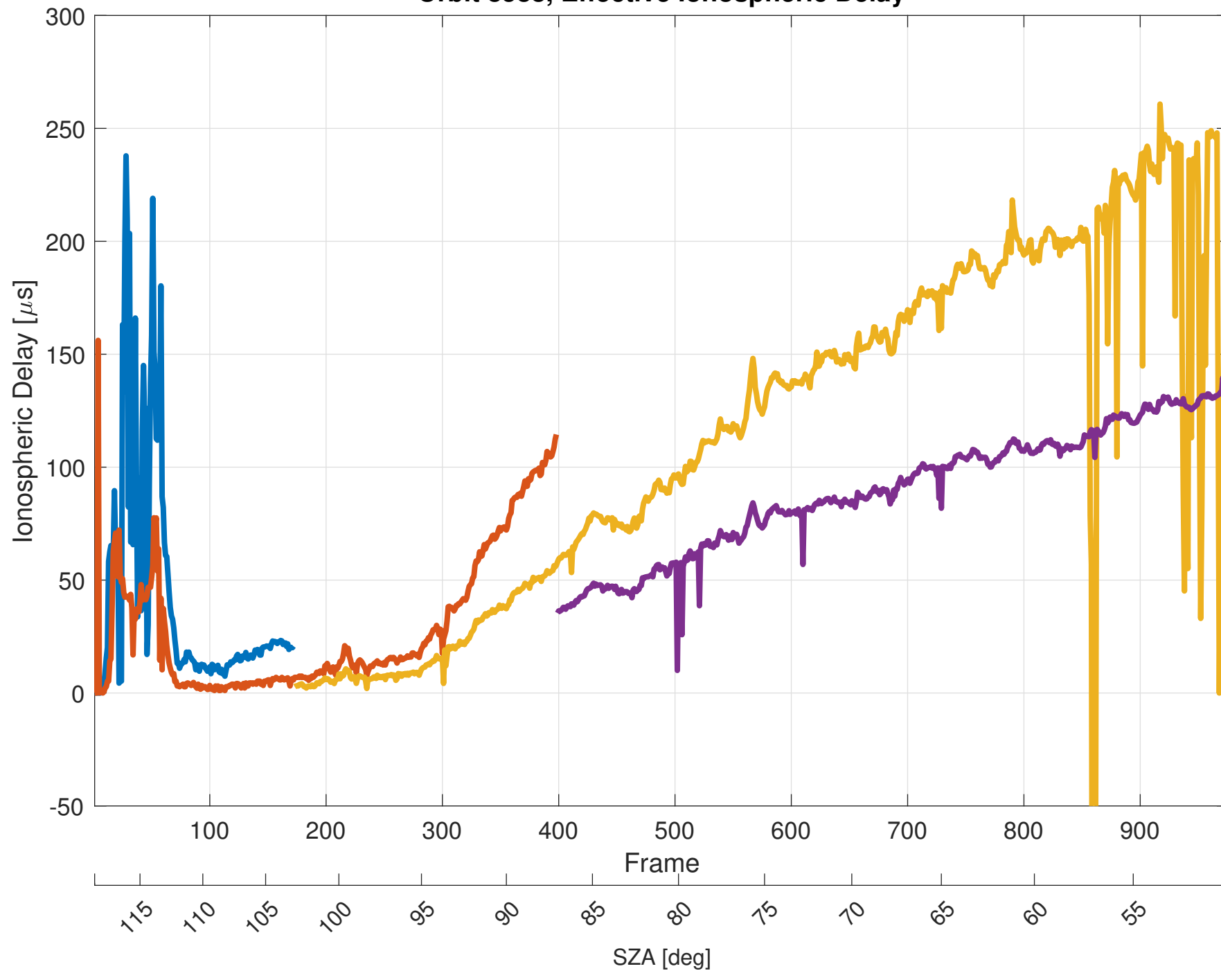
Orbit 8588, Effective Ionospheric Delay
