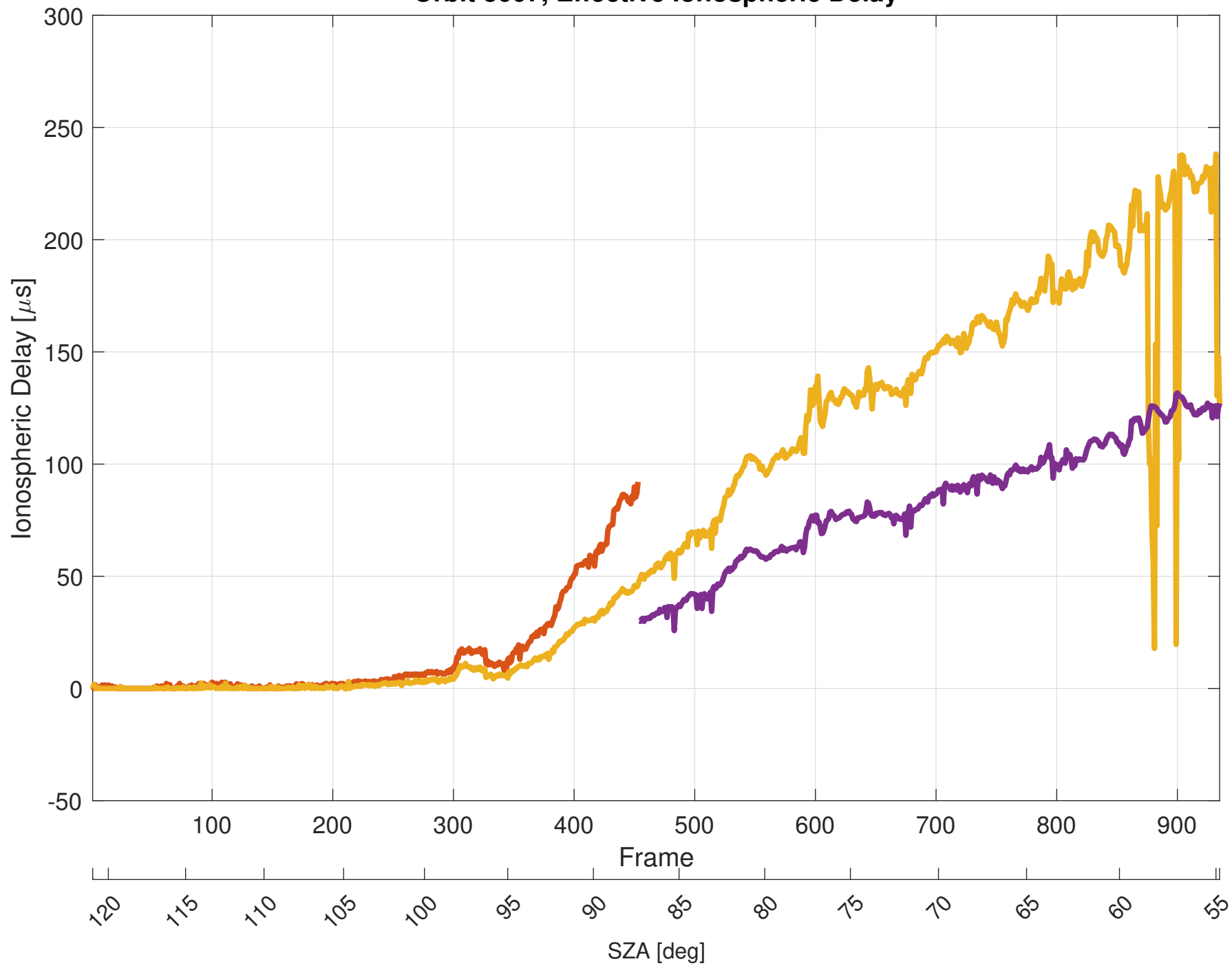
Orbit 8607, Effective Ionospheric Delay
