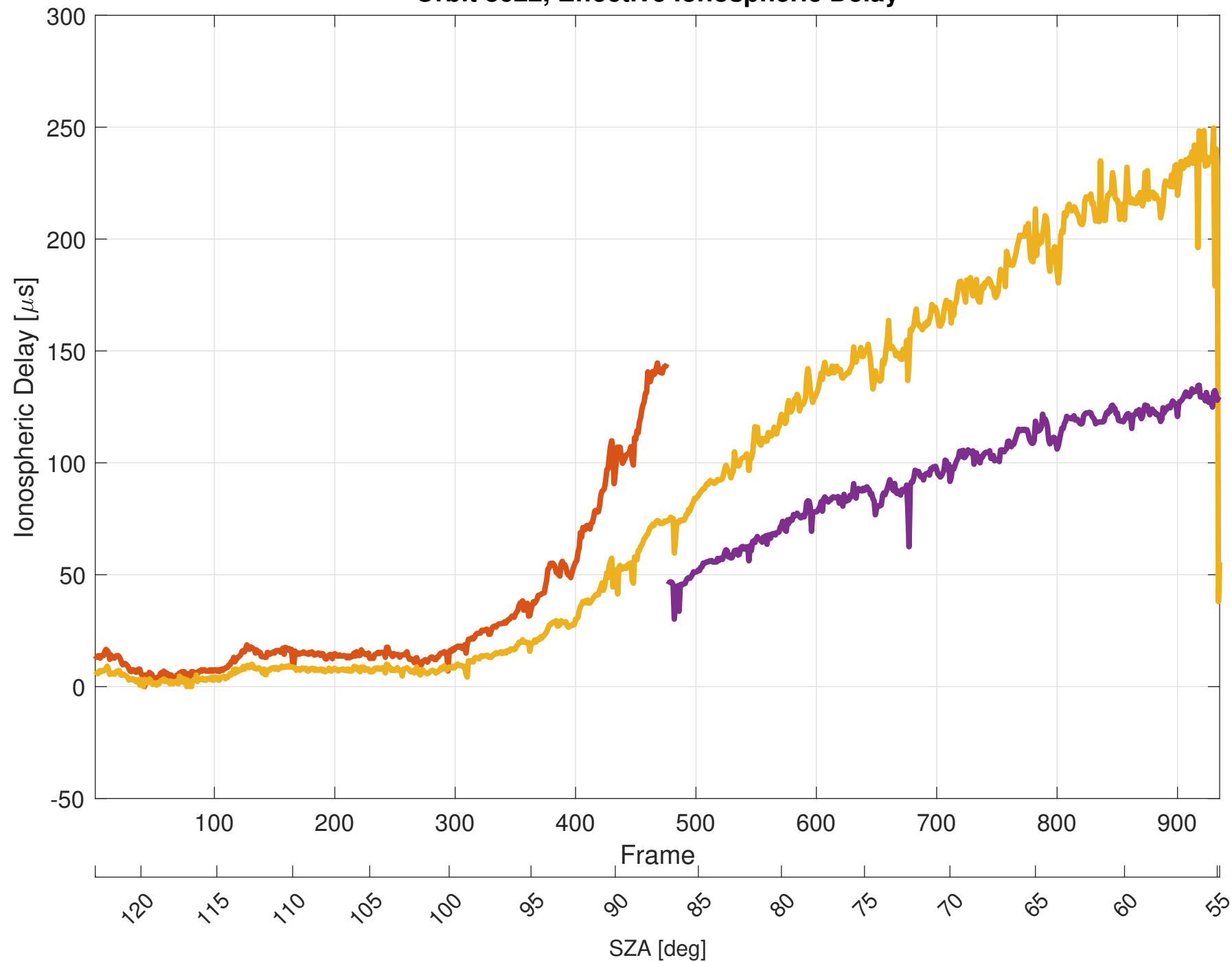
Orbit 8622, Effective Ionospheric Delay
