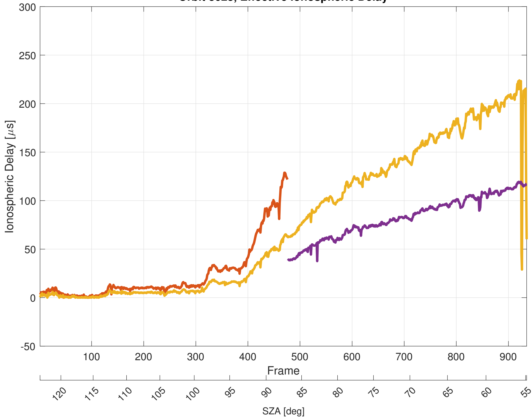
Orbit 8623, Effective Ionospheric Delay
