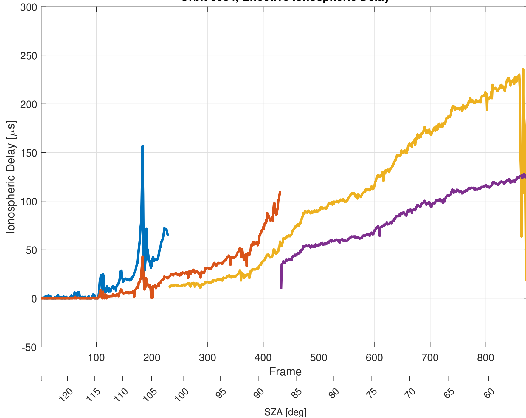
Orbit 8634, Effective Ionospheric Delay
