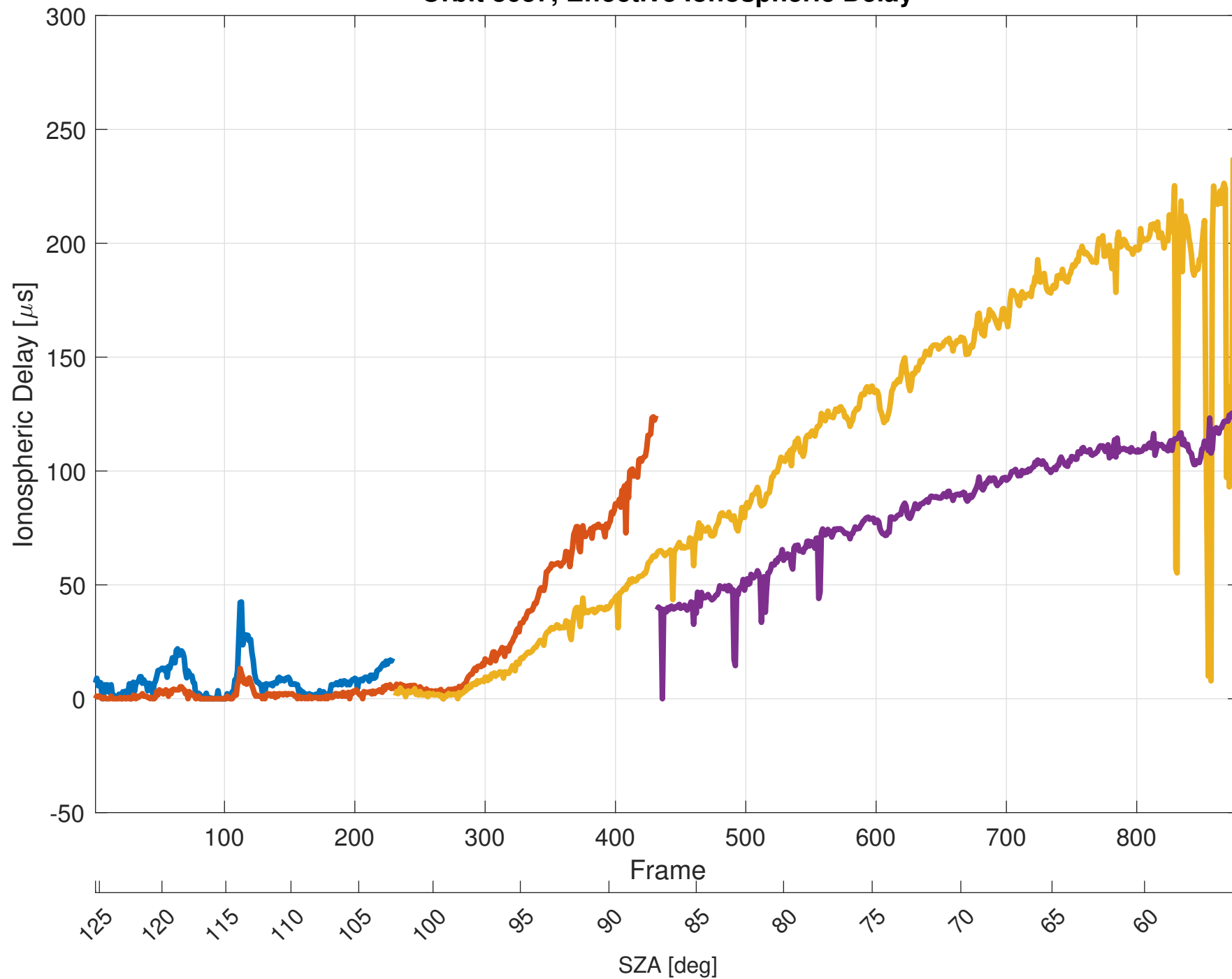
Orbit 8637, Effective Ionospheric Delay
