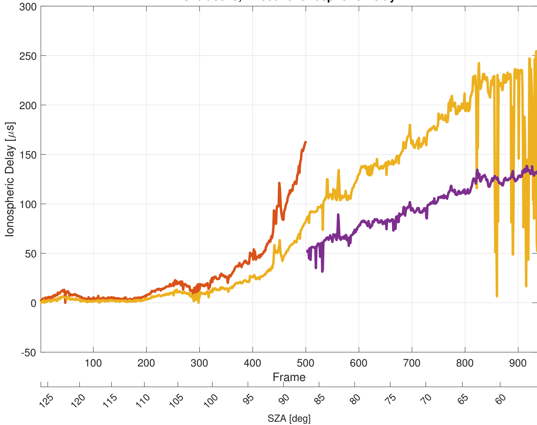
Orbit 8643, Effective Ionospheric Delay
