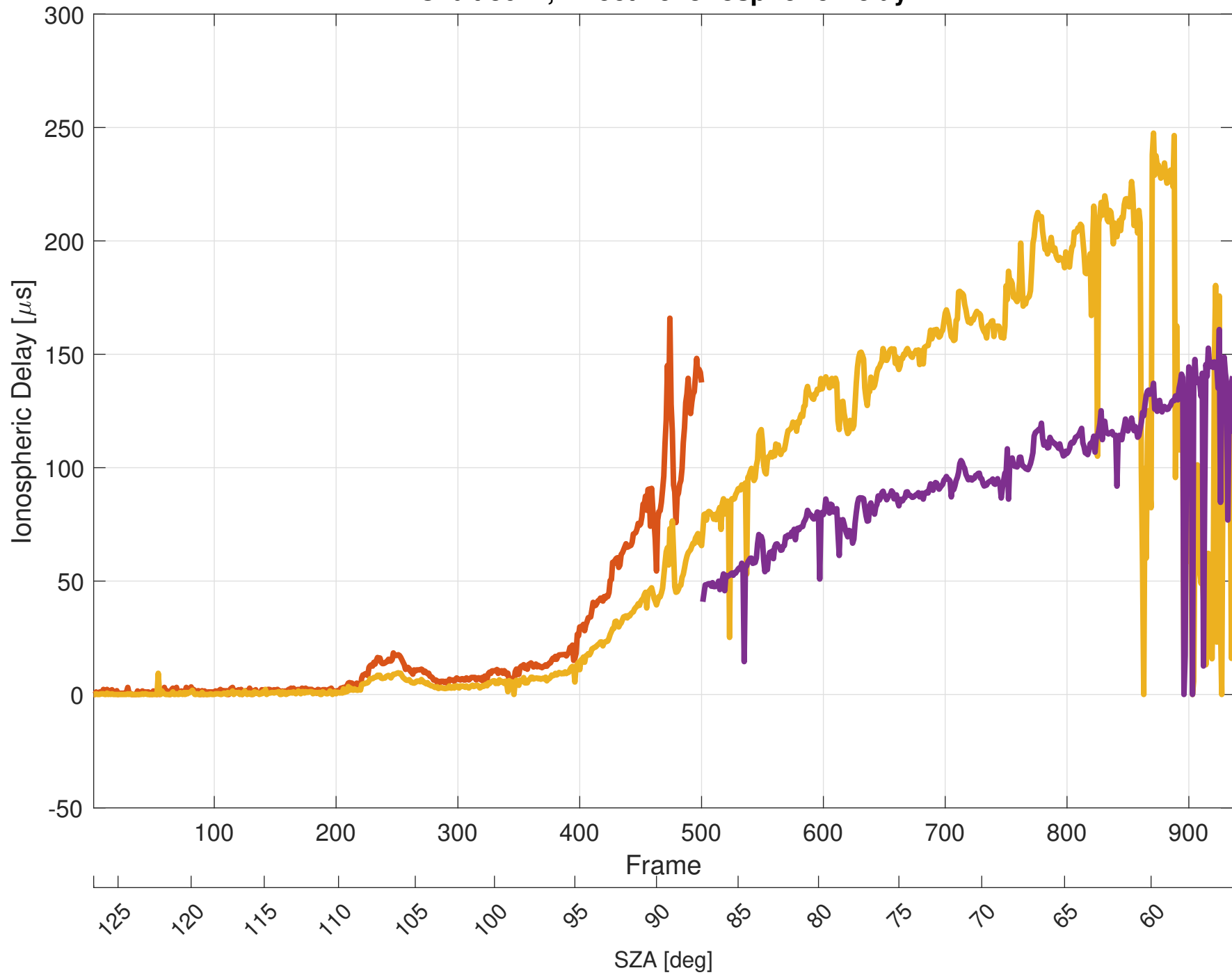
Orbit 8647, Effective Ionospheric Delay
