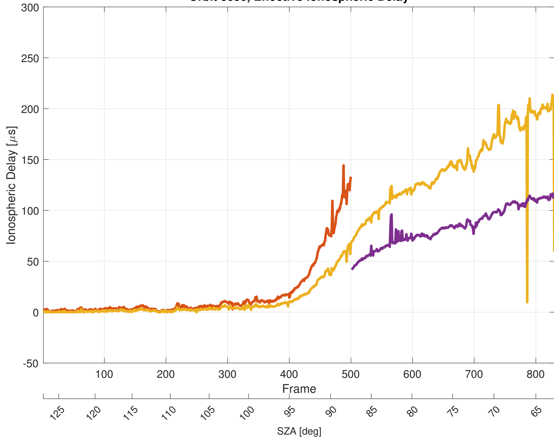
Orbit 8650, Effective Ionospheric Delay
