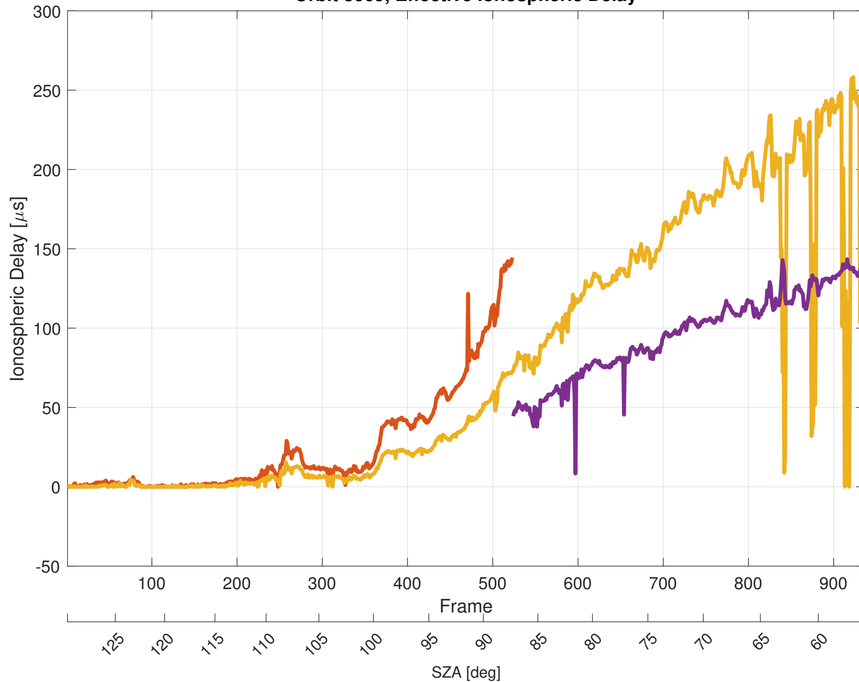
Orbit 8669, Effective Ionospheric Delay
