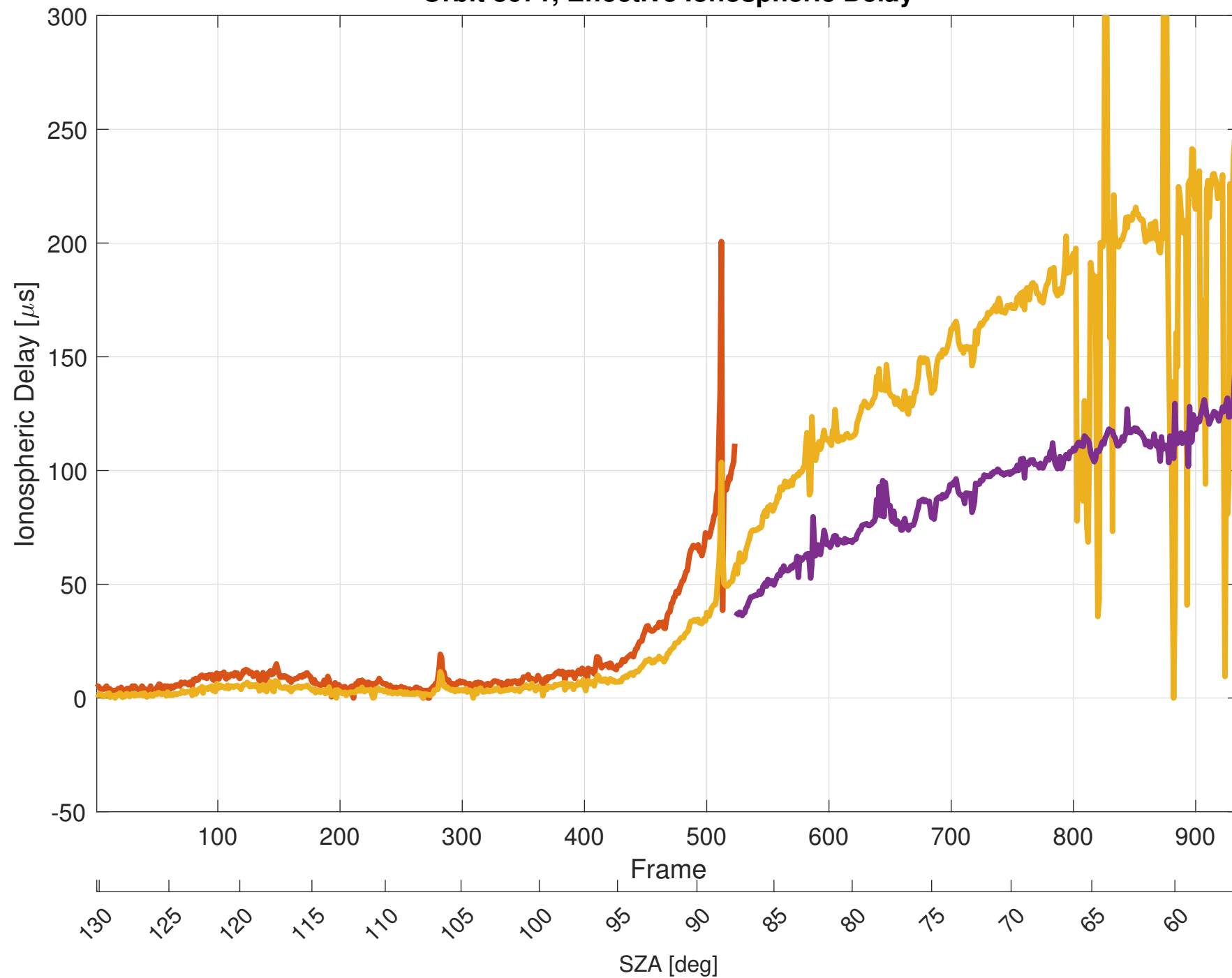
Orbit 8671, Effective Ionospheric Delay
