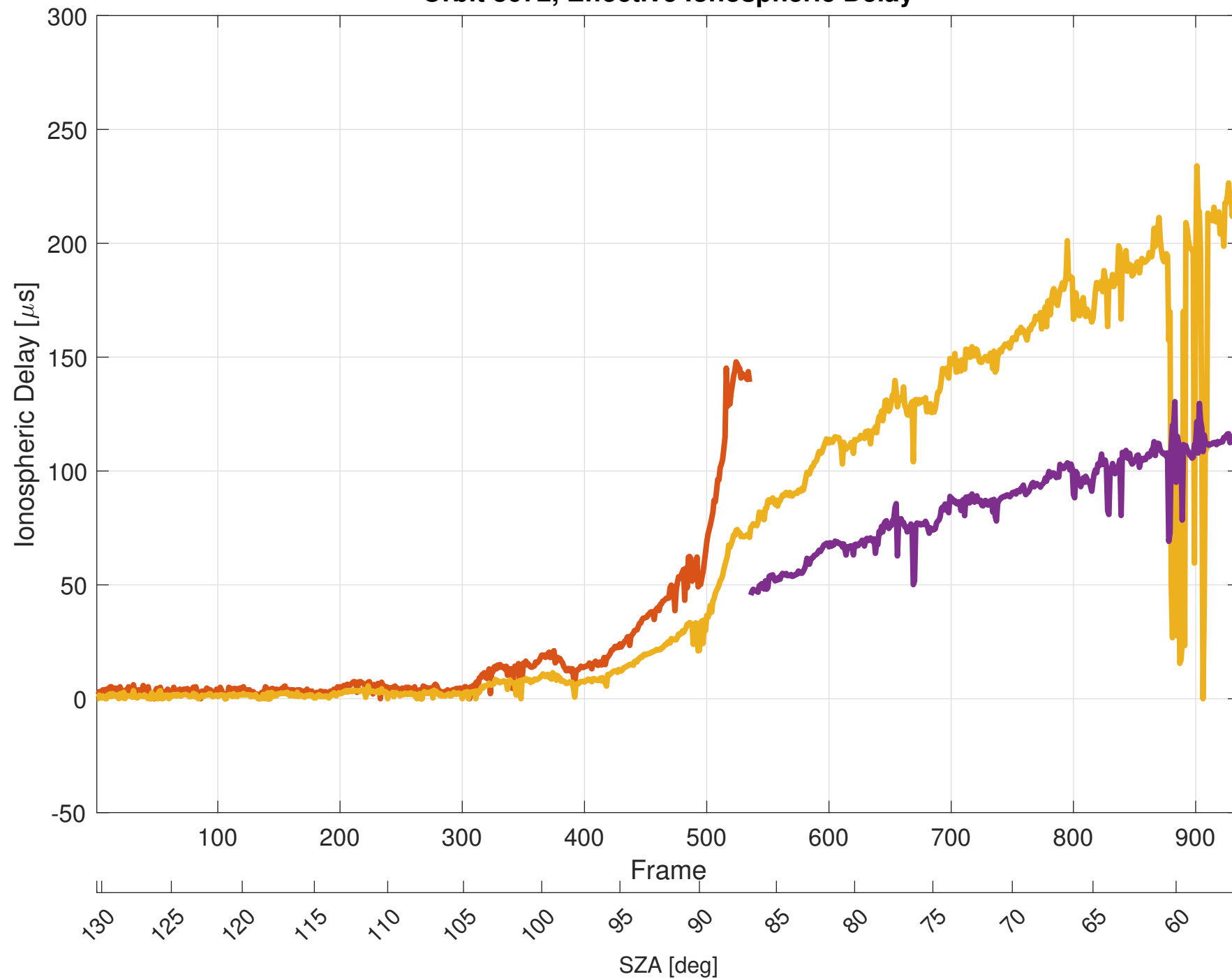
Orbit 8672, Effective Ionospheric Delay
