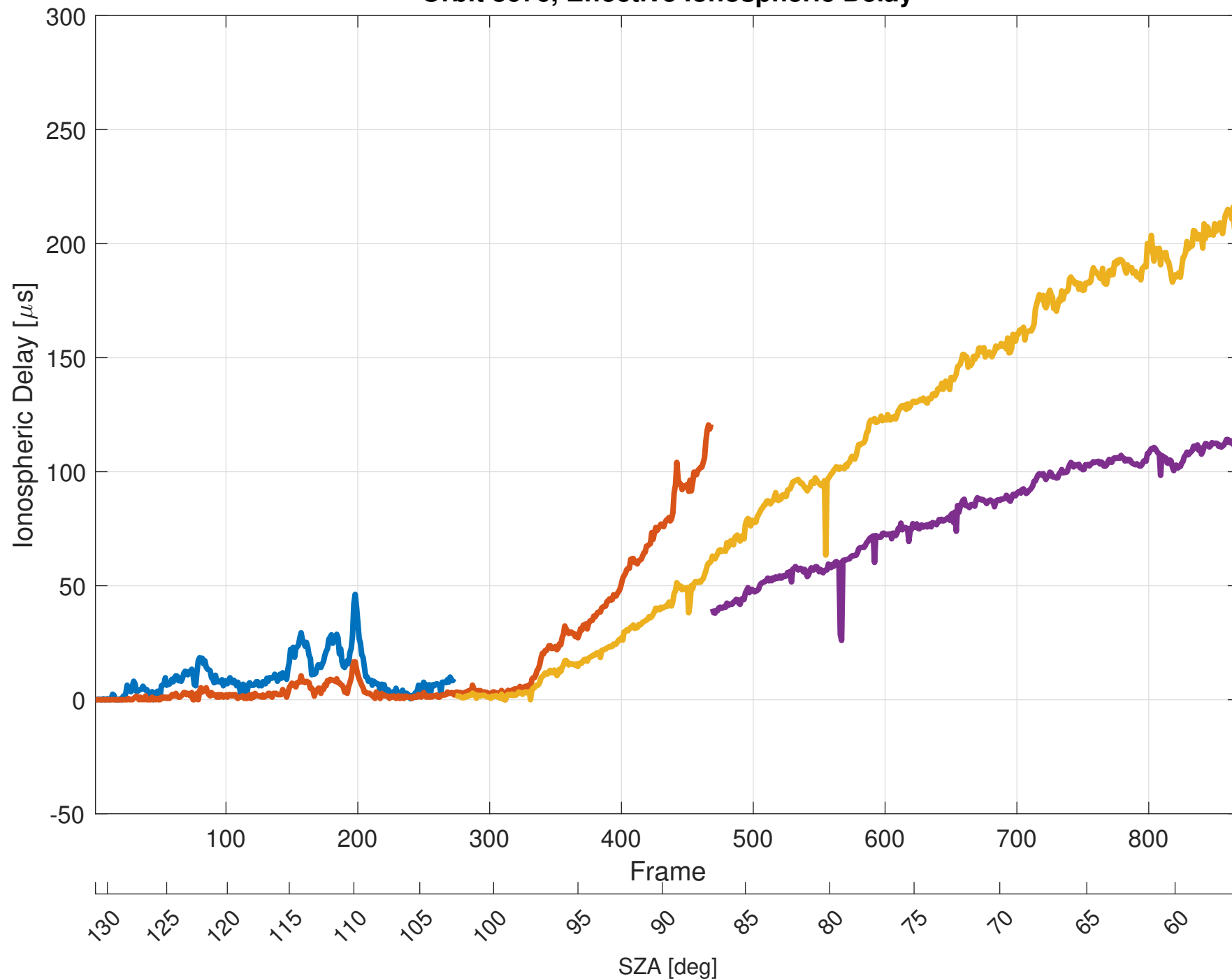
Orbit 8676, Effective Ionospheric Delay
