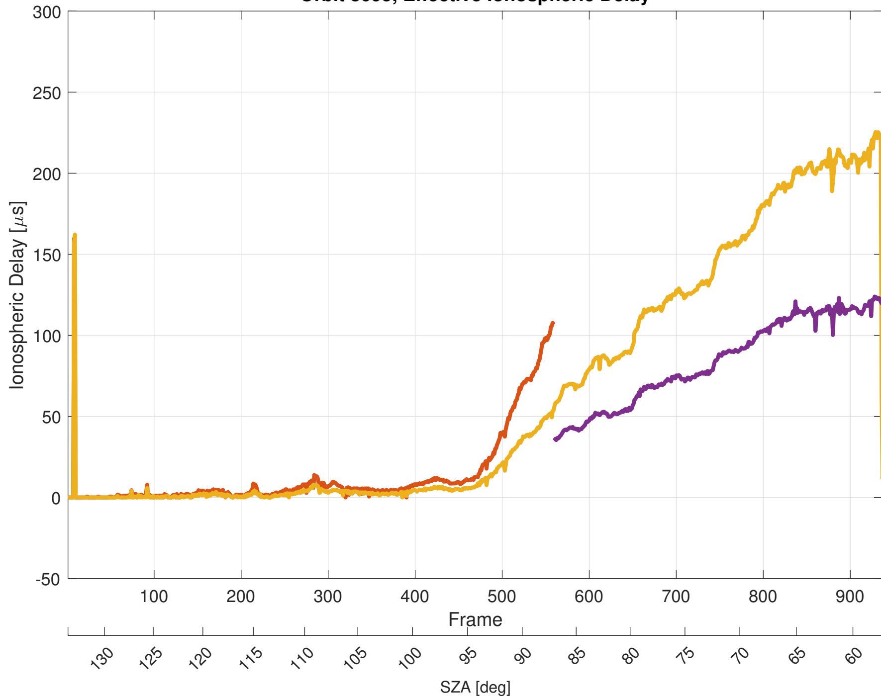
Orbit 8695, Effective Ionospheric Delay
