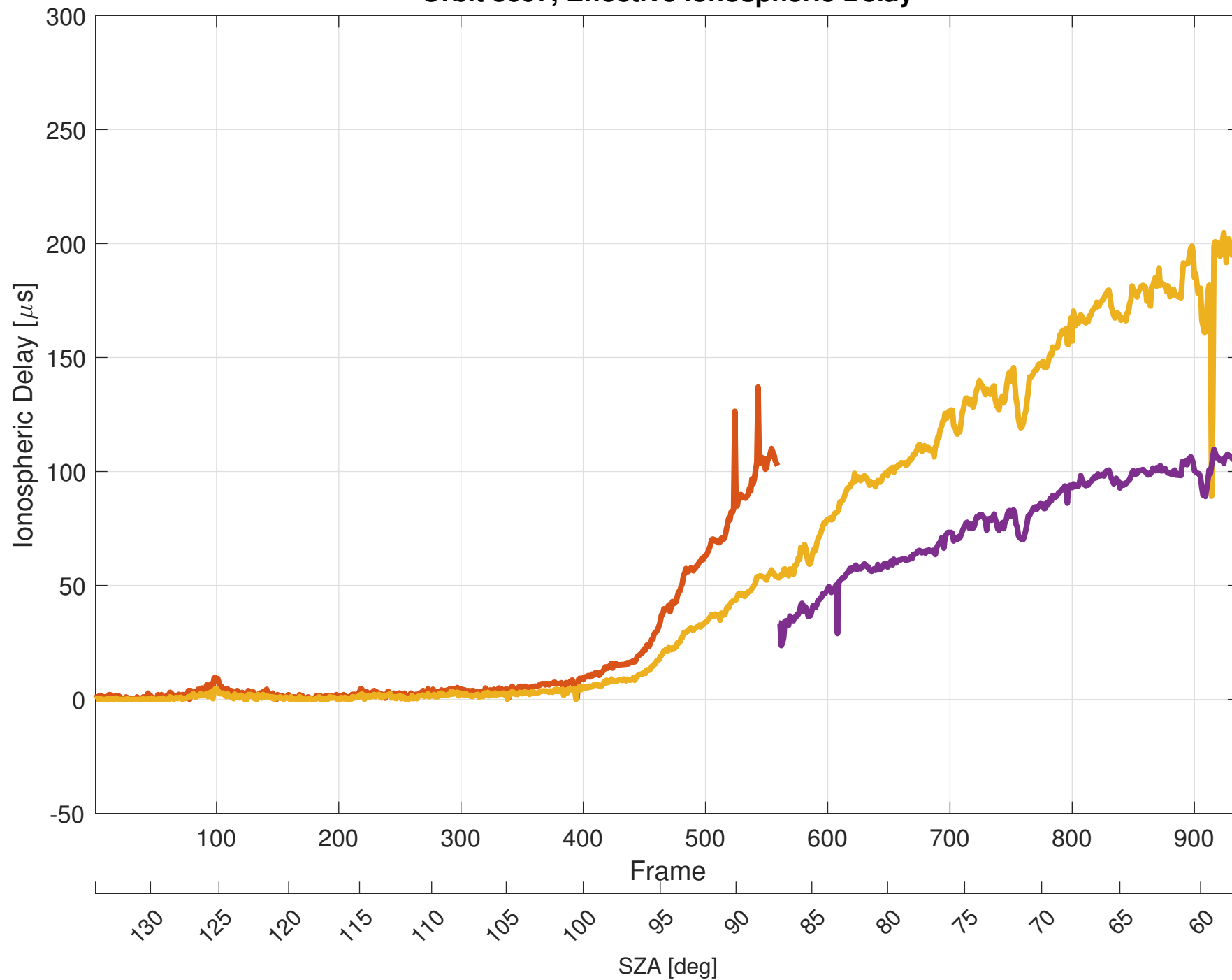
Orbit 8697, Effective Ionospheric Delay
