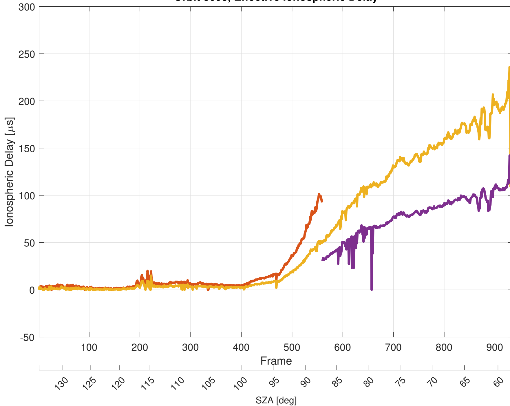
Orbit 8698, Effective Ionospheric Delay
