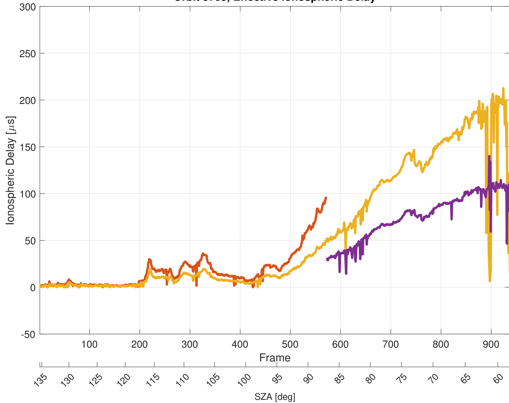
Orbit 8705, Effective Ionospheric Delay
