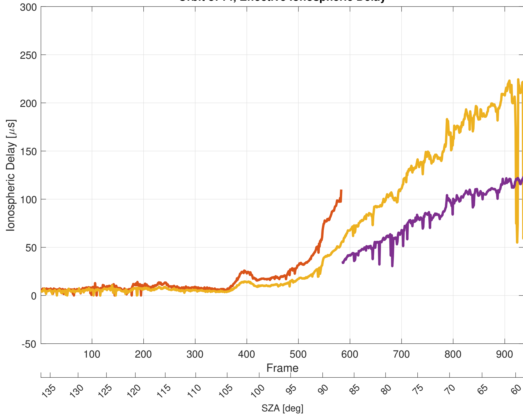
Orbit 8714, Effective Ionospheric Delay
