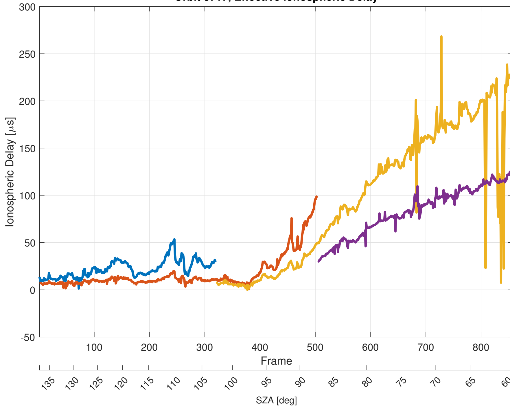
Orbit 8717, Effective Ionospheric Delay
