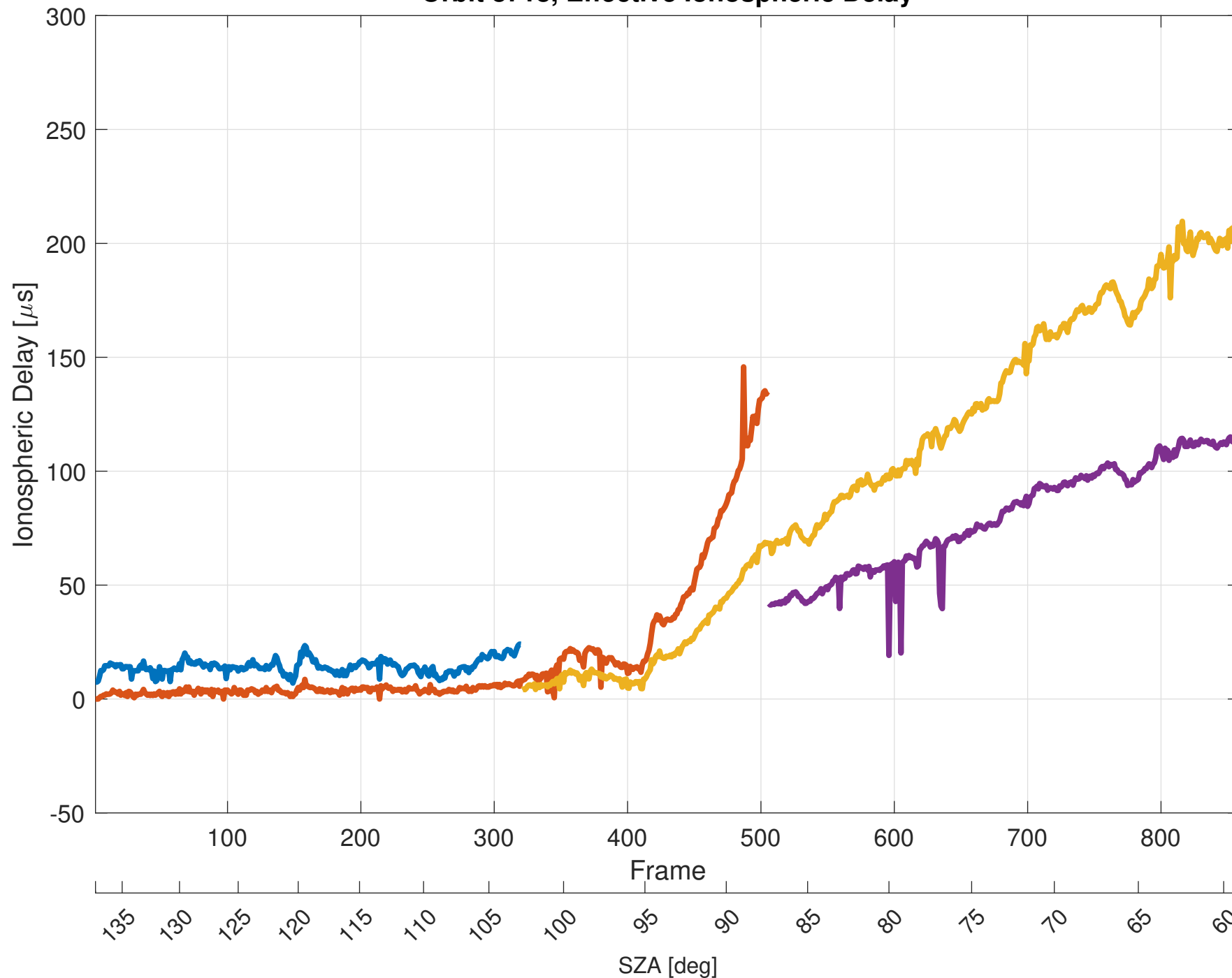
Orbit 8718, Effective Ionospheric Delay
