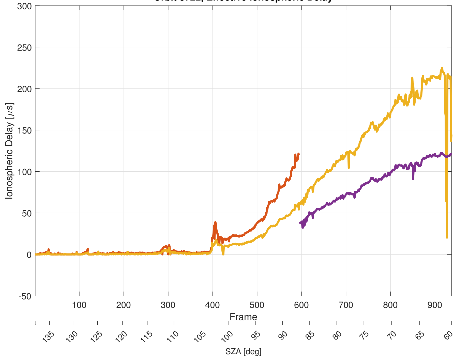
Orbit 8722, Effective Ionospheric Delay
