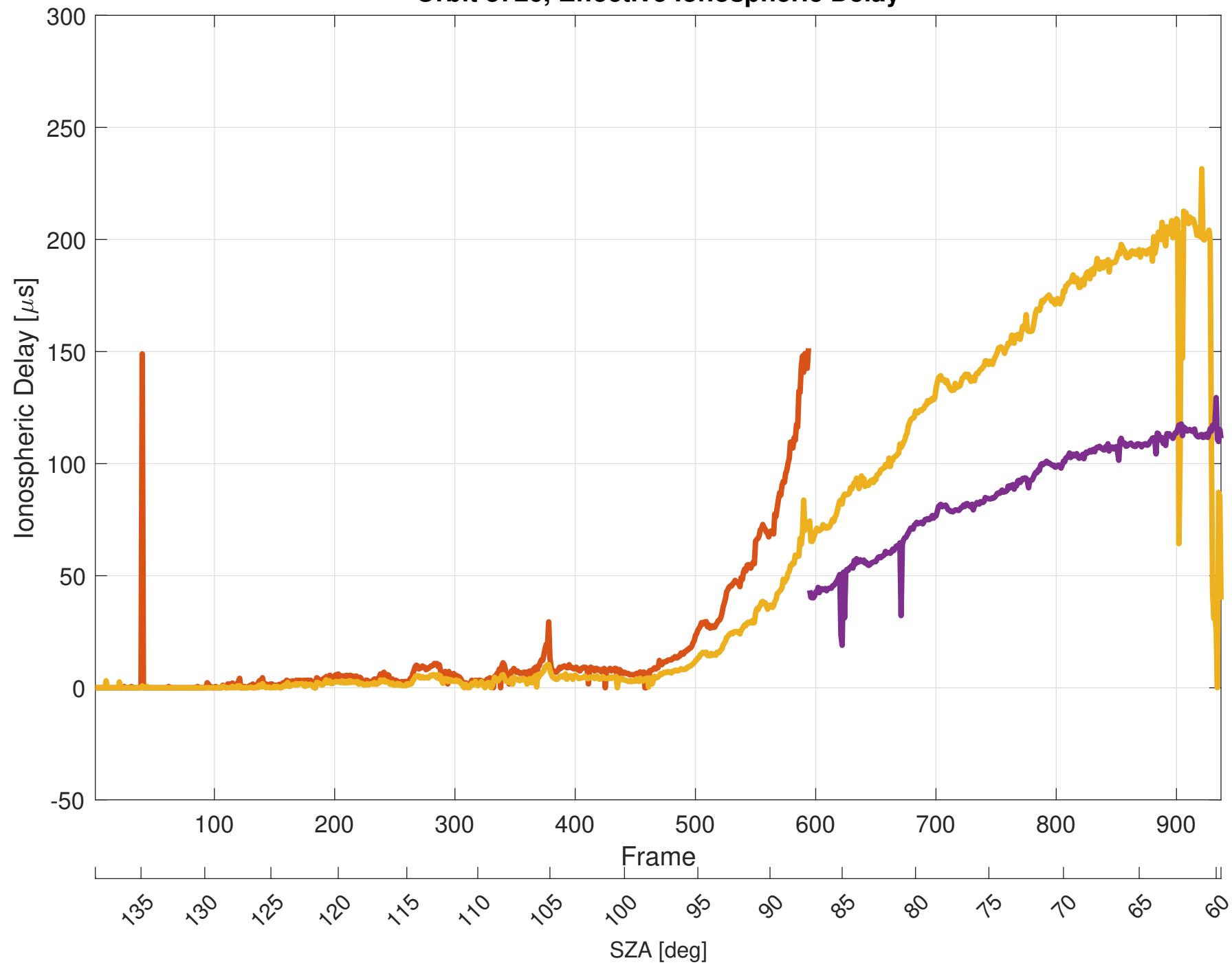
Orbit 8726, Effective Ionospheric Delay
