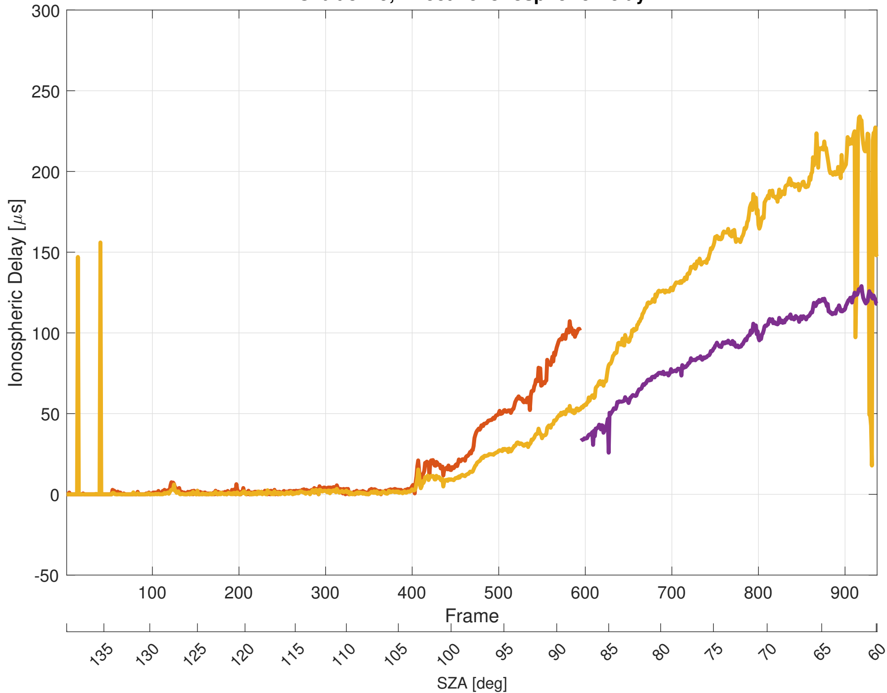
Orbit 8729, Effective Ionospheric Delay
