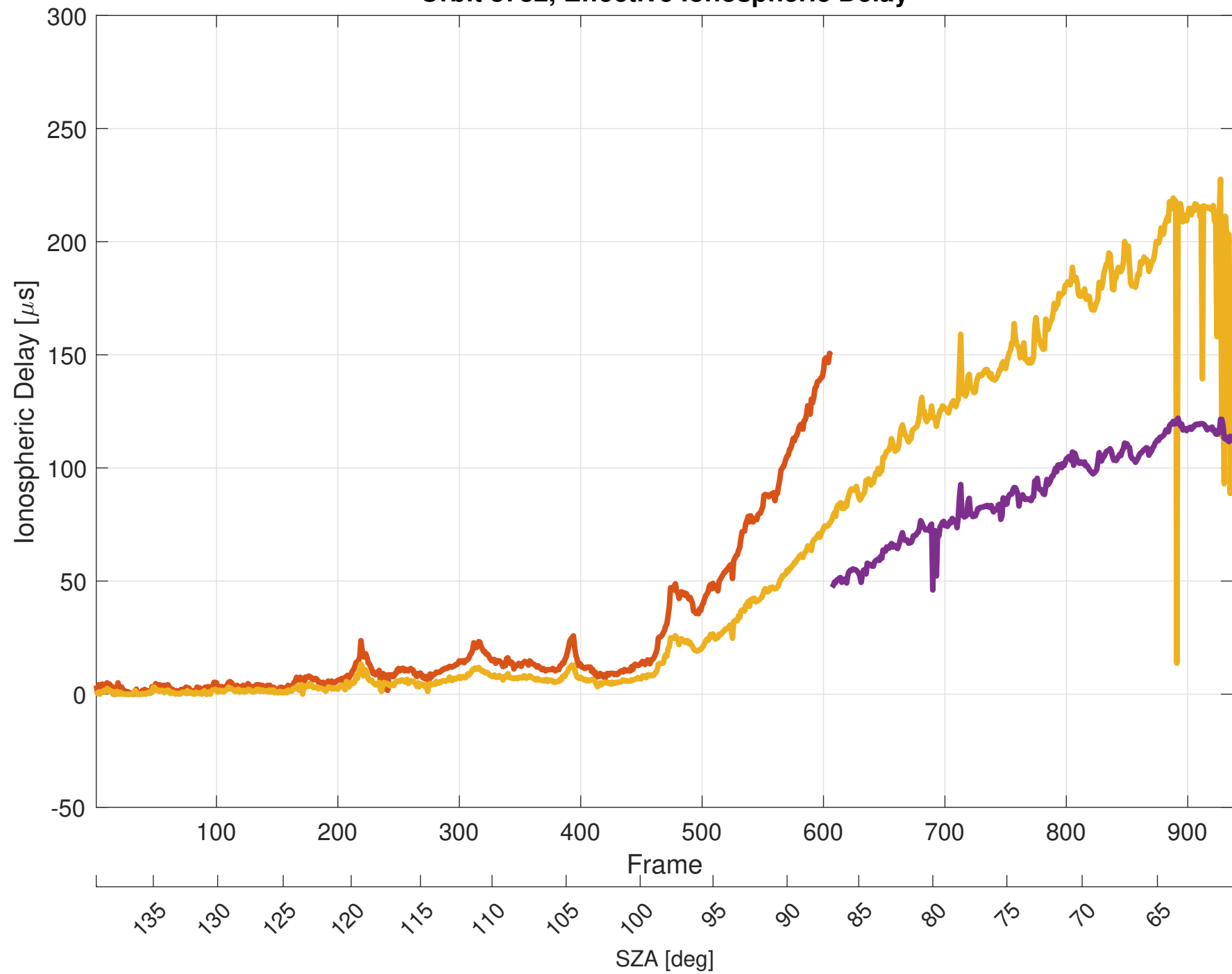
Orbit 8732, Effective Ionospheric Delay
