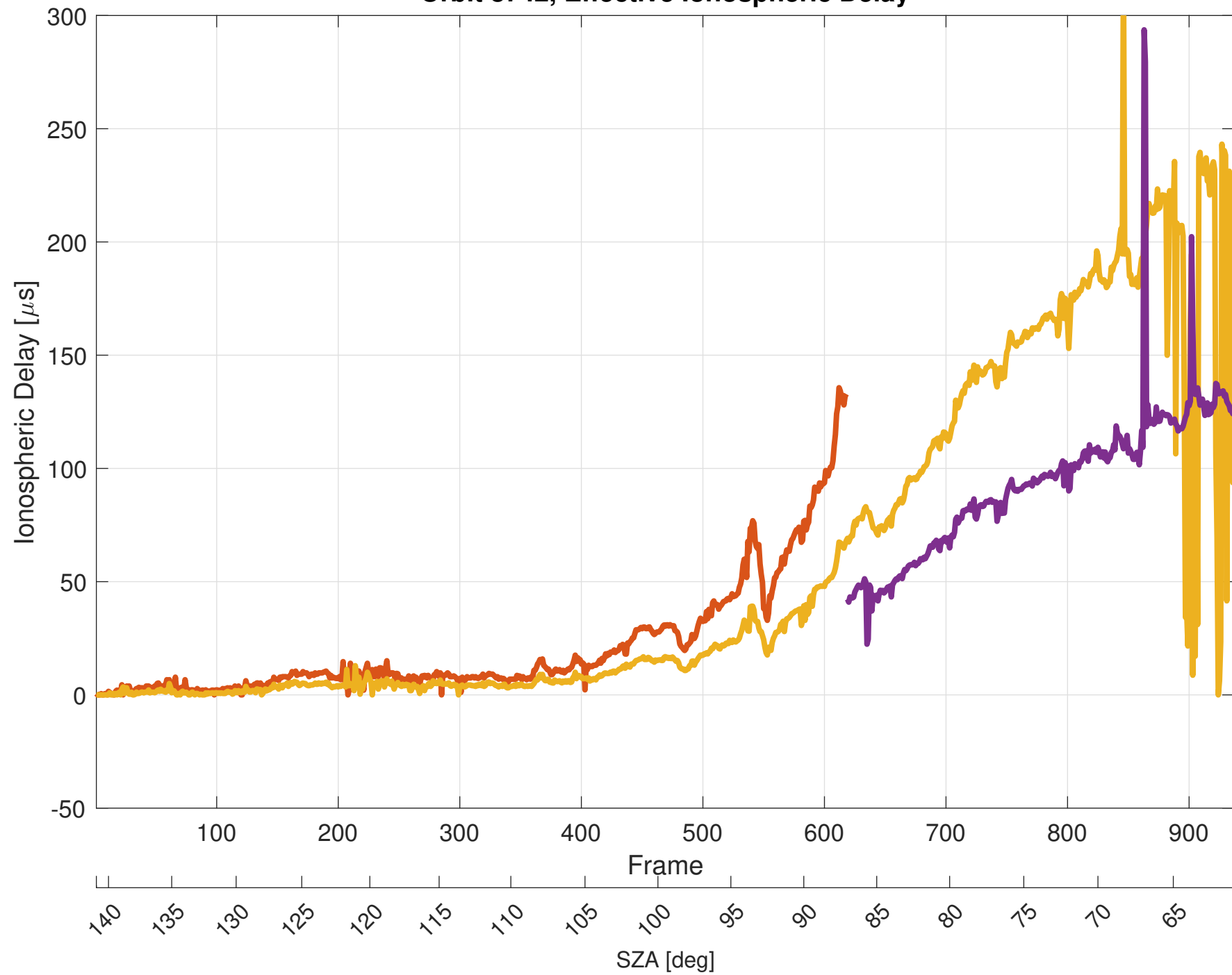
Orbit 8742, Effective Ionospheric Delay
