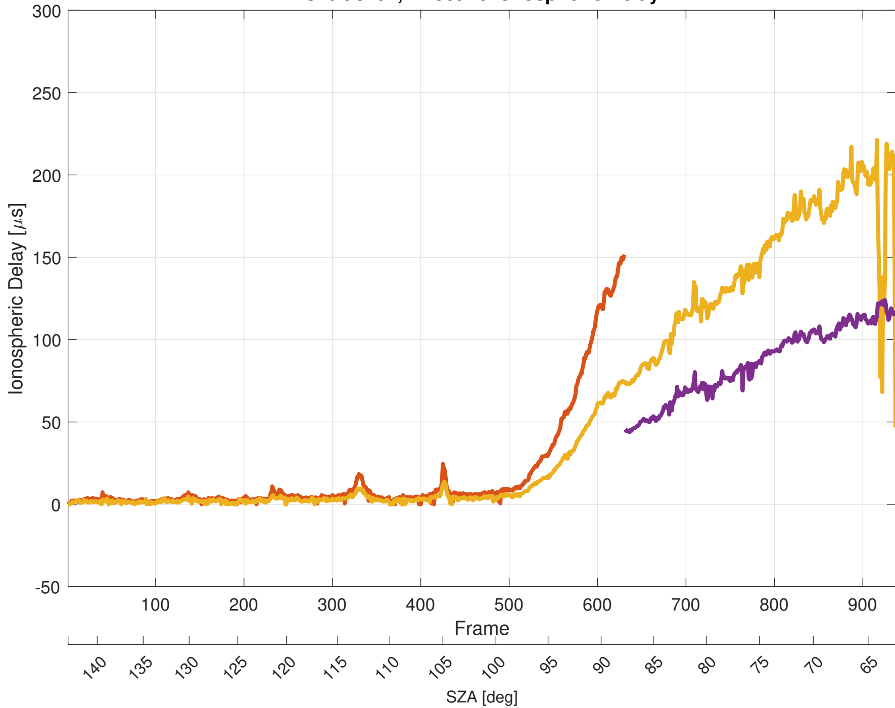
Orbit 8757, Effective Ionospheric Delay
