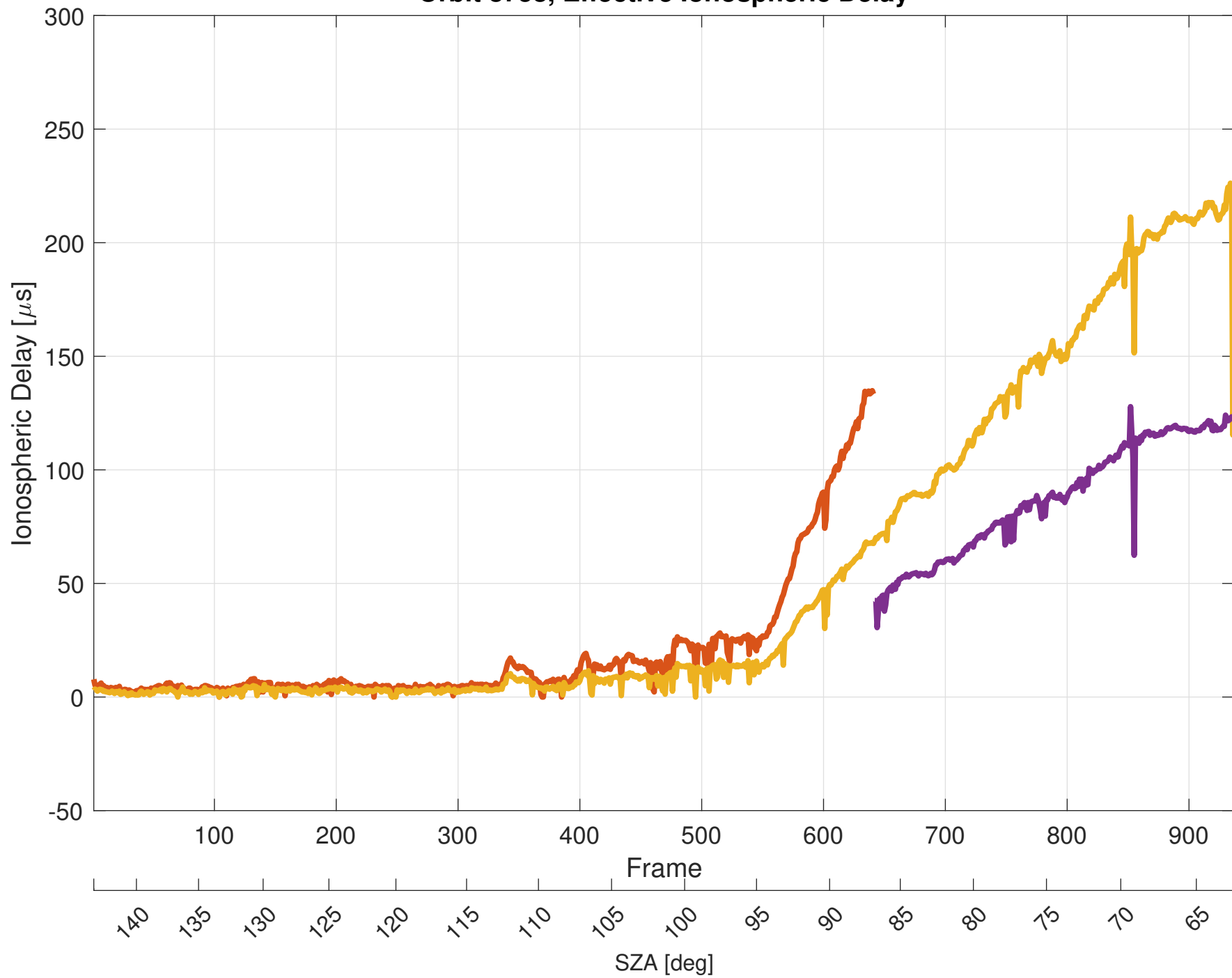
Orbit 8758, Effective Ionospheric Delay
