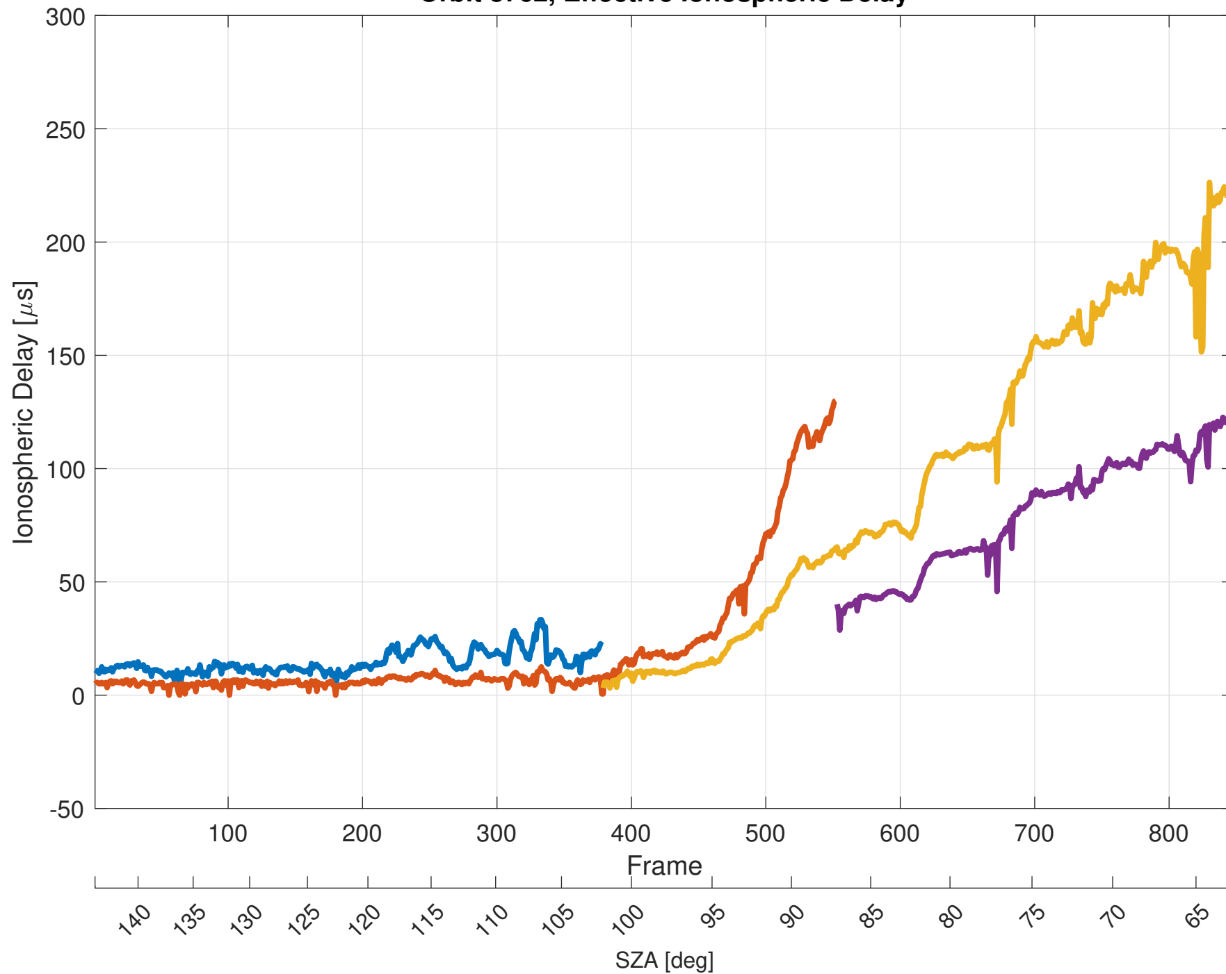
Orbit 8762, Effective Ionospheric Delay
