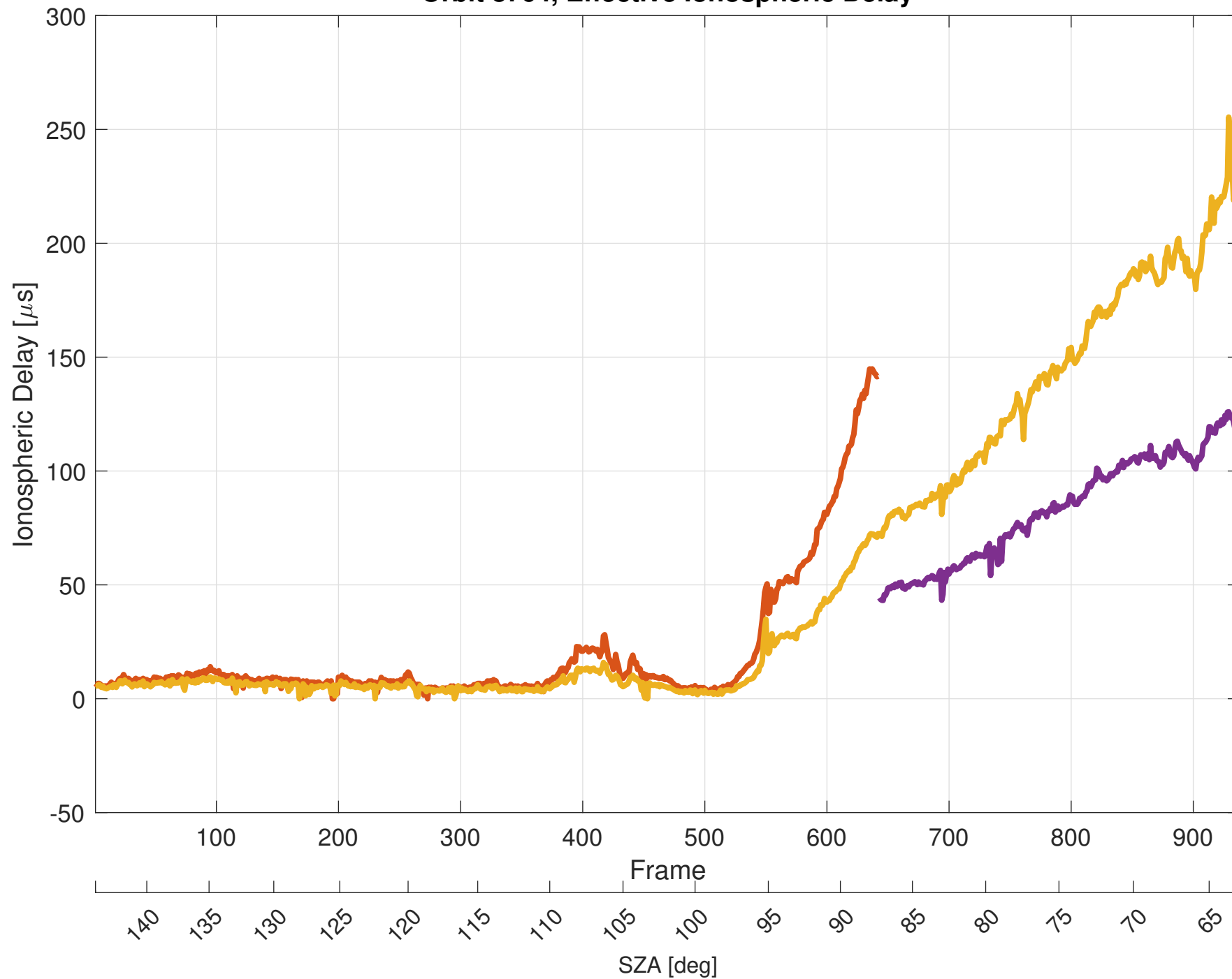
Orbit 8764, Effective Ionospheric Delay
