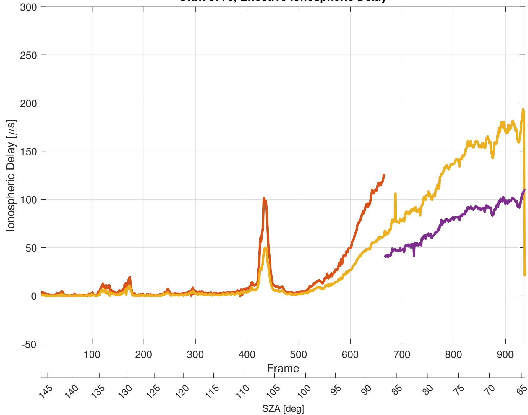
Orbit 8778, Effective Ionospheric Delay
