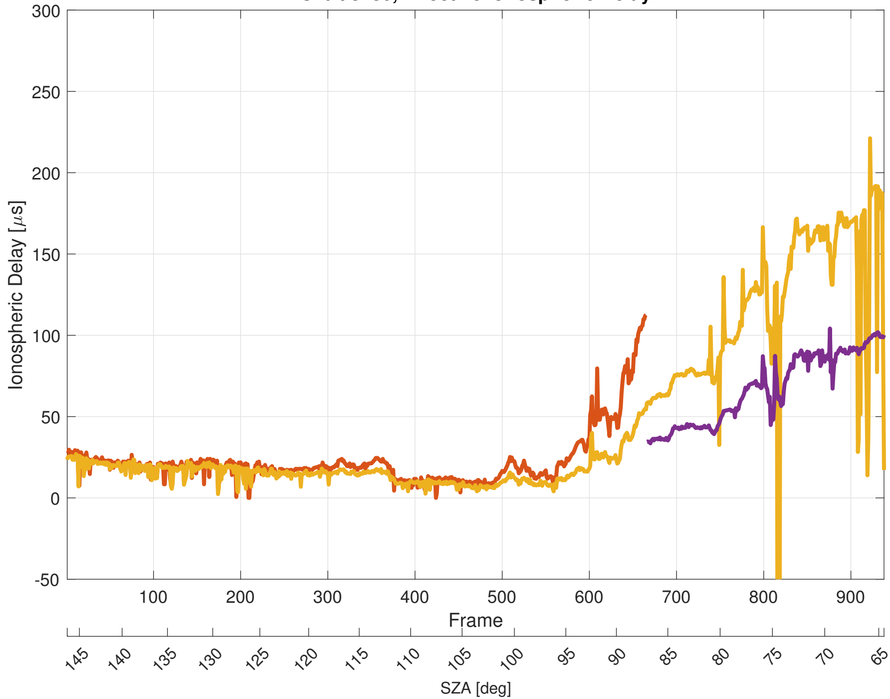
Orbit 8780, Effective Ionospheric Delay
