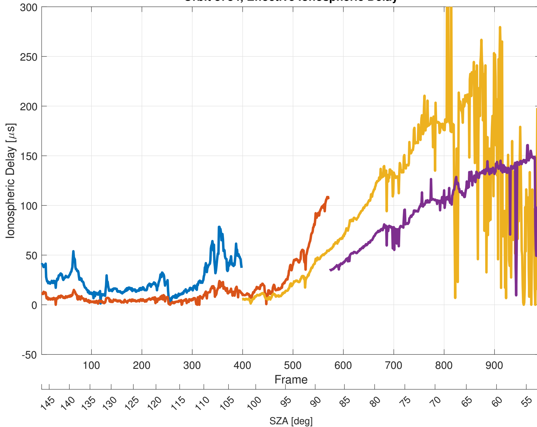
Orbit 8784, Effective Ionospheric Delay
