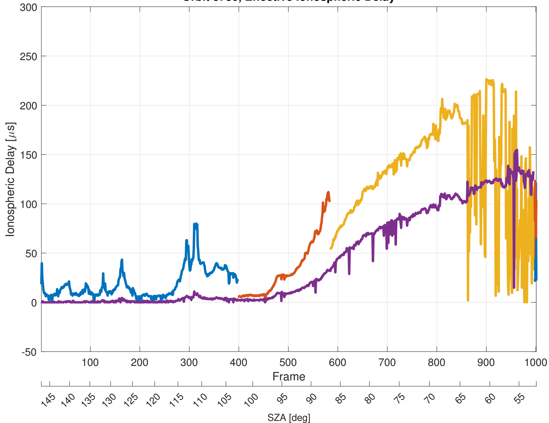
Orbit 8786, Effective Ionospheric Delay
