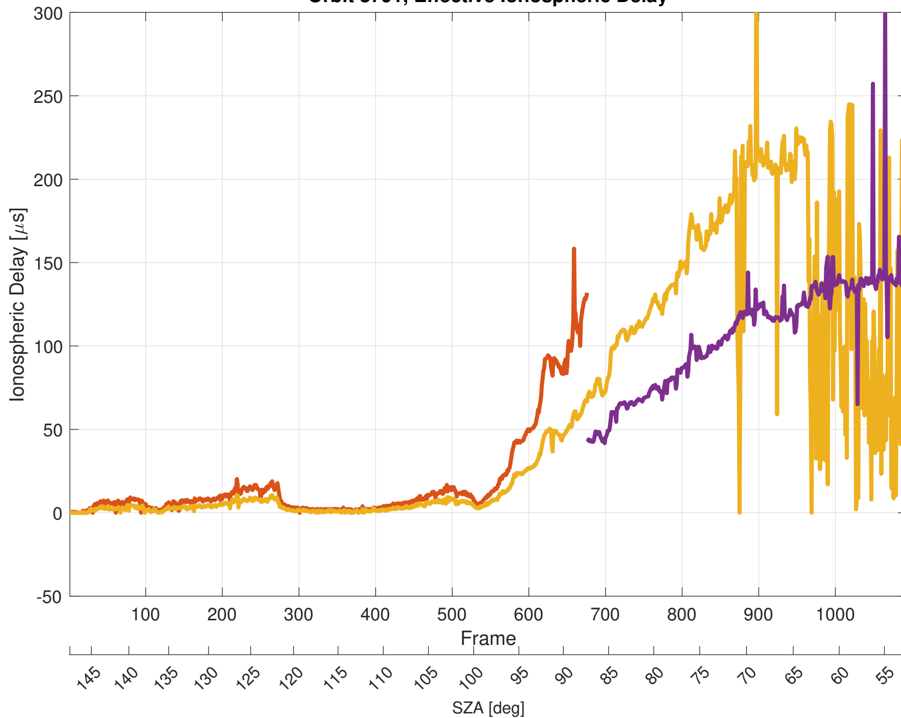
Orbit 8791, Effective Ionospheric Delay
