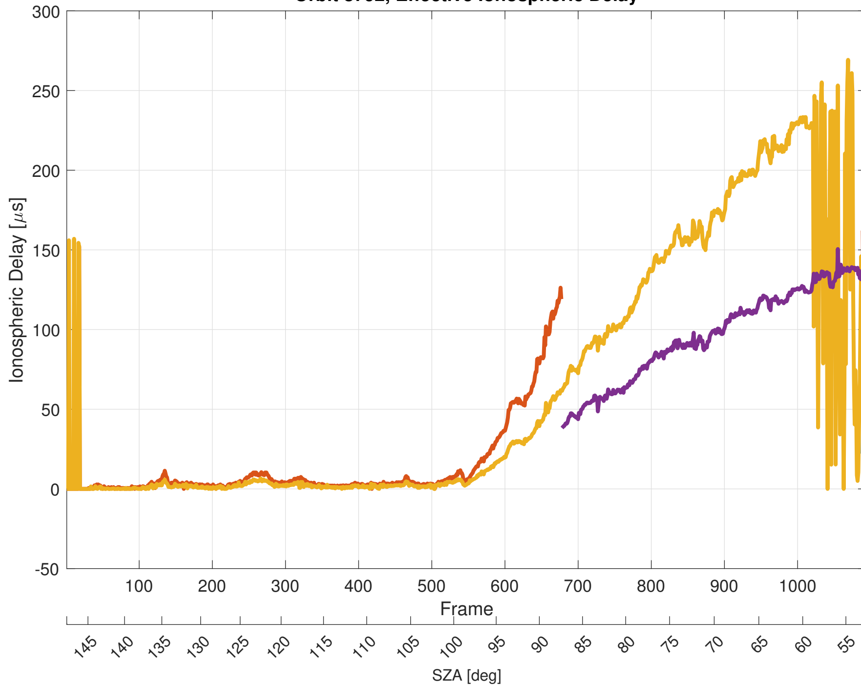
Orbit 8792, Effective Ionospheric Delay
