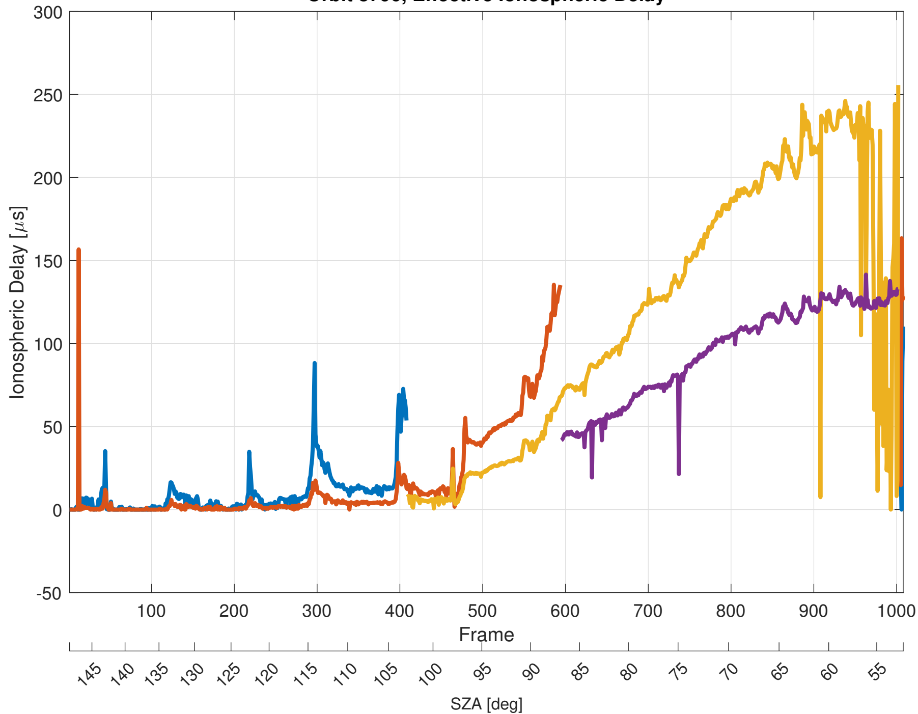
Orbit 8796, Effective Ionospheric Delay
