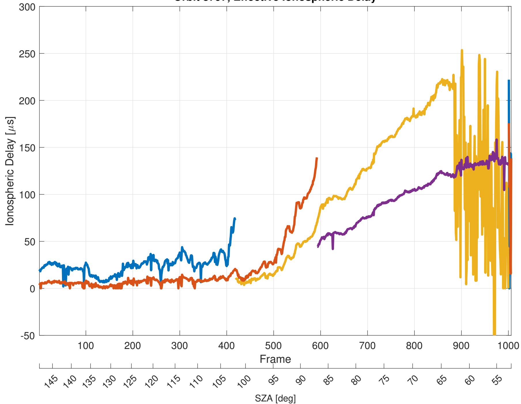
Orbit 8797, Effective Ionospheric Delay
