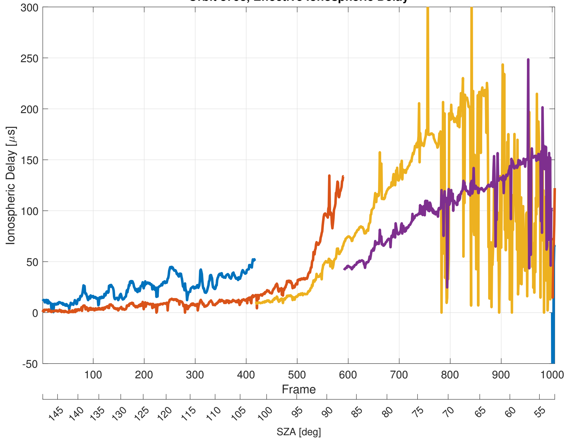
Orbit 8798, Effective Ionospheric Delay
