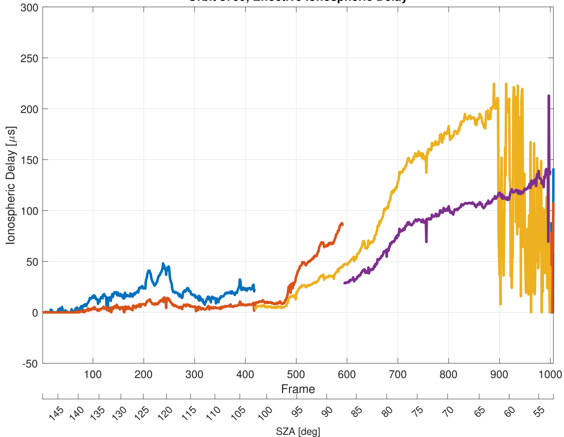
Orbit 8799, Effective Ionospheric Delay
