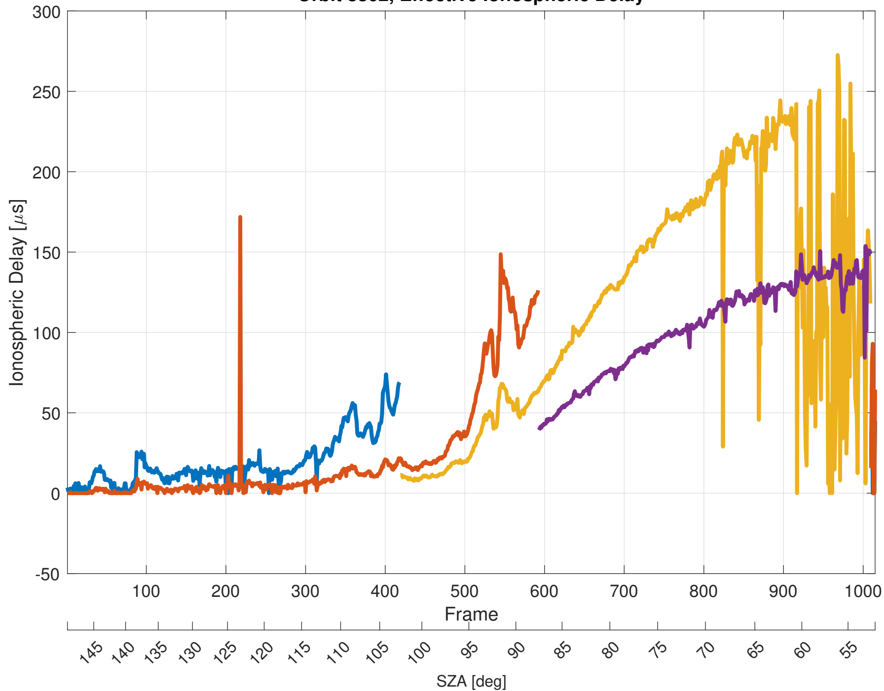
Orbit 8802, Effective Ionospheric Delay
