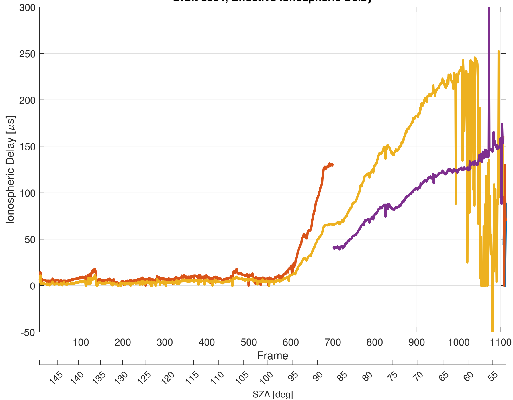
Orbit 8804, Effective Ionospheric Delay
