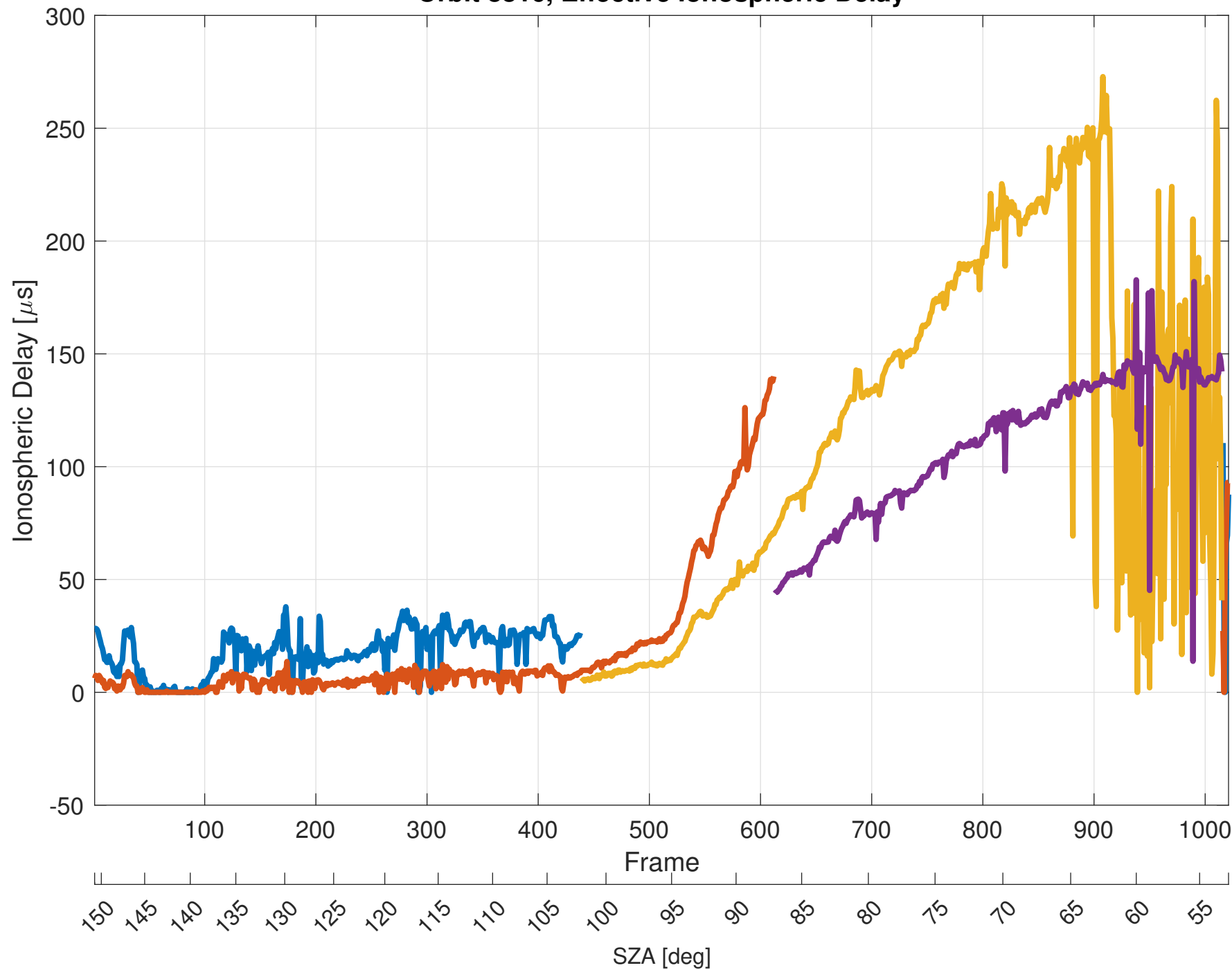
Orbit 8816, Effective Ionospheric Delay
